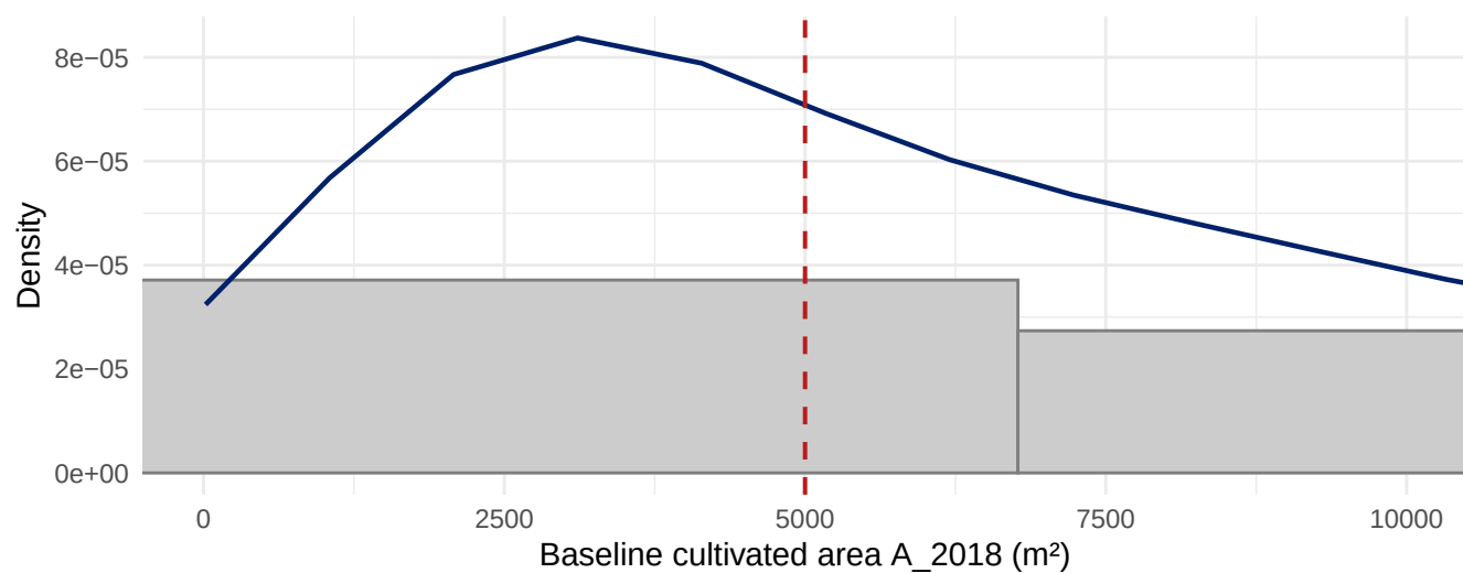
(a) Cultivated area (cutoff 5,000 m 2 ); t=0.68, p=0.499
