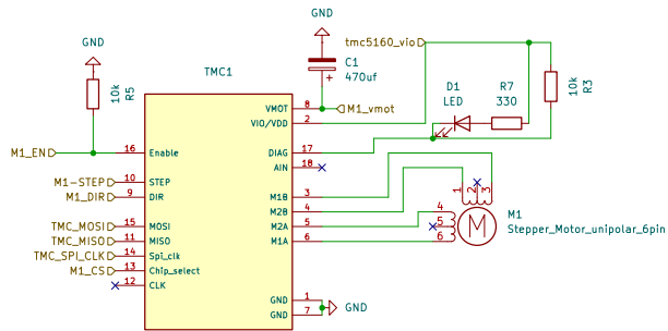
M1_control with TMC2240/TMC5160
