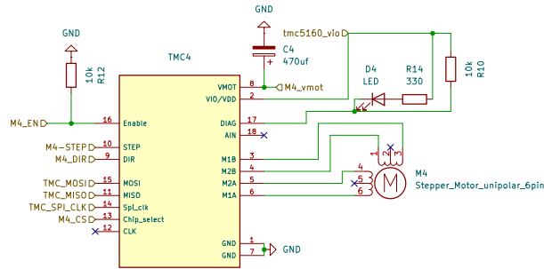
M4_control with TMC2240/TMC5160
