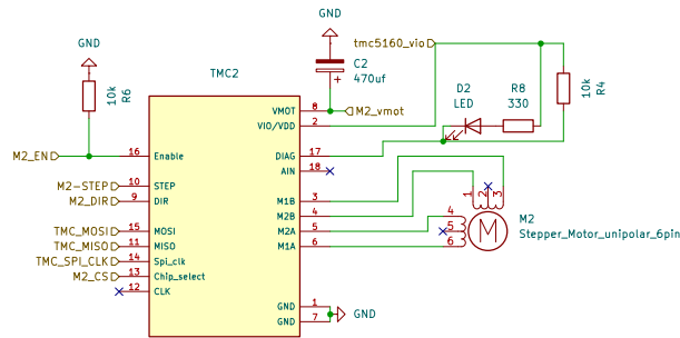
M2_control with TMC2240/TMC5160
