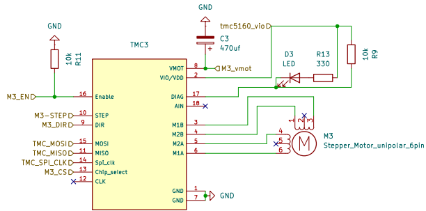
M3_control with TMC2240/TMC5160
