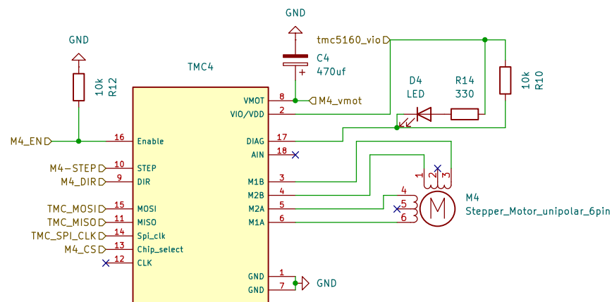
M4_control with TMC2240/TMC5160
