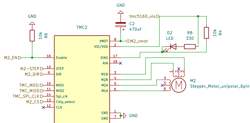
M2_control with TMC2240/TMC5160
