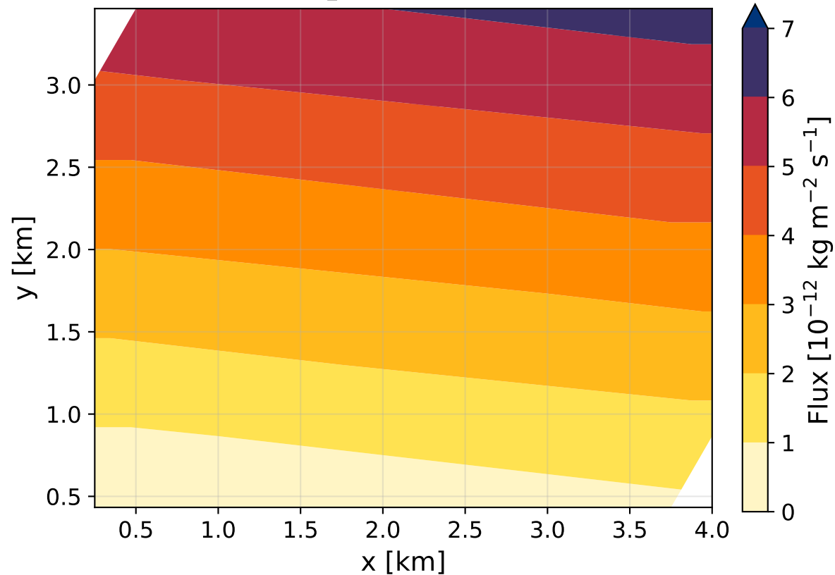
NO 2 surface flux
