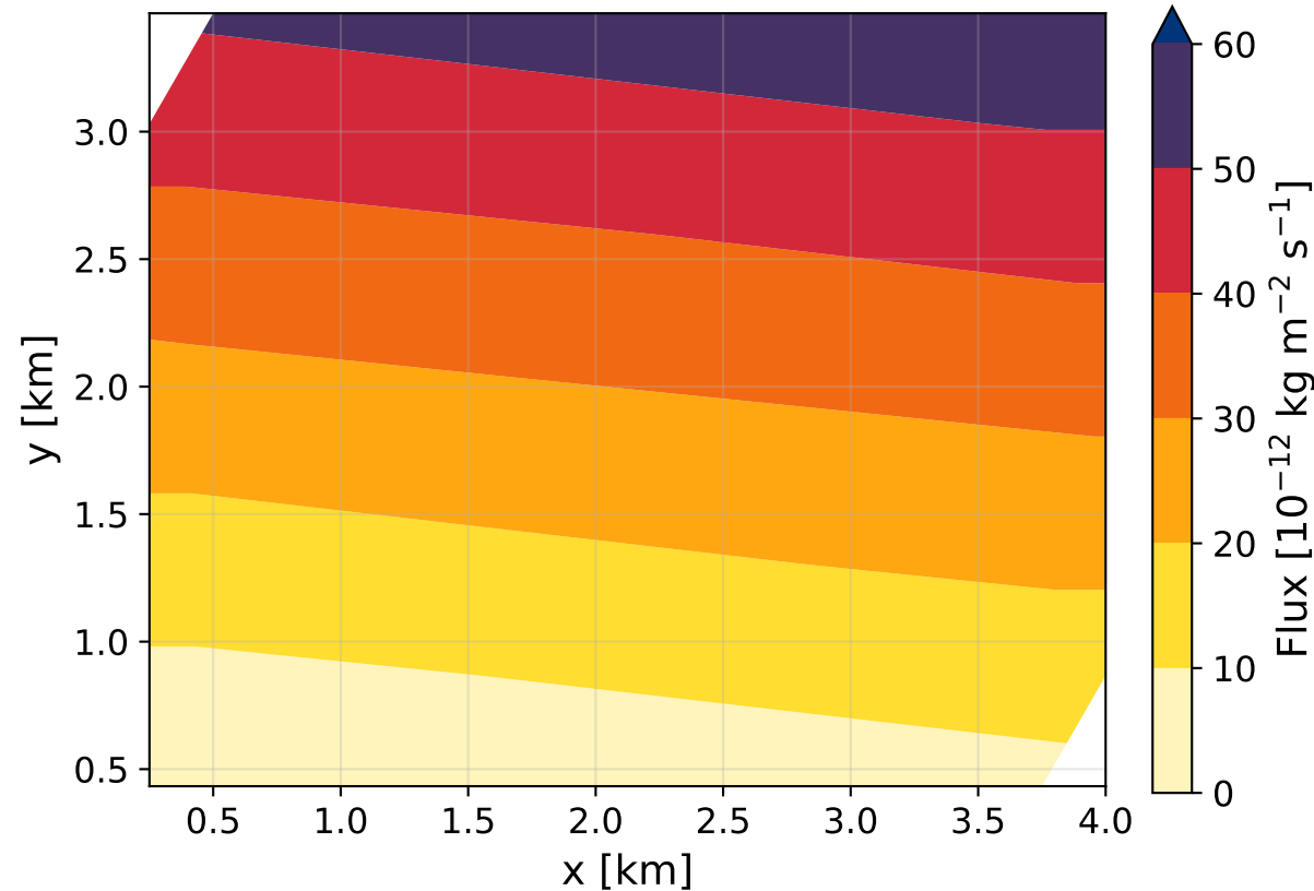
NO surface flux
