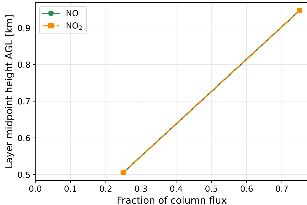
Normalized elevated-source allocation
