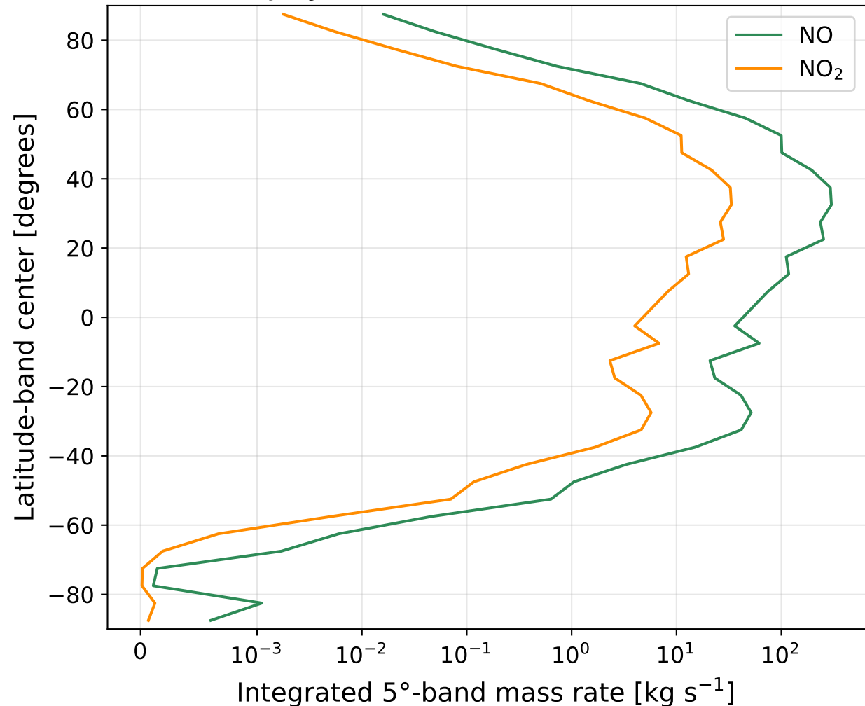
July zonal source distribution
