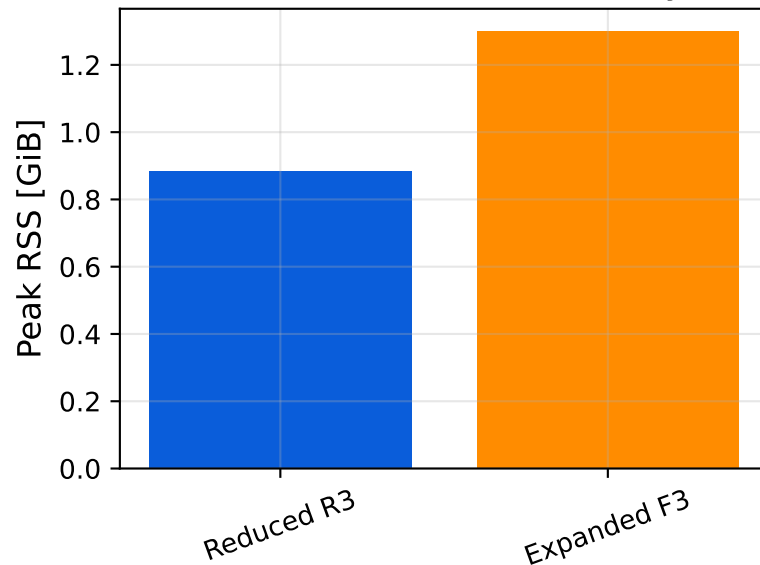
(b) Peak resident memory
