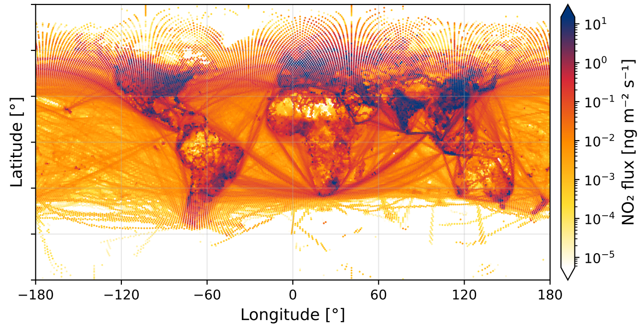
(b) Applied NO 2 mass flux
