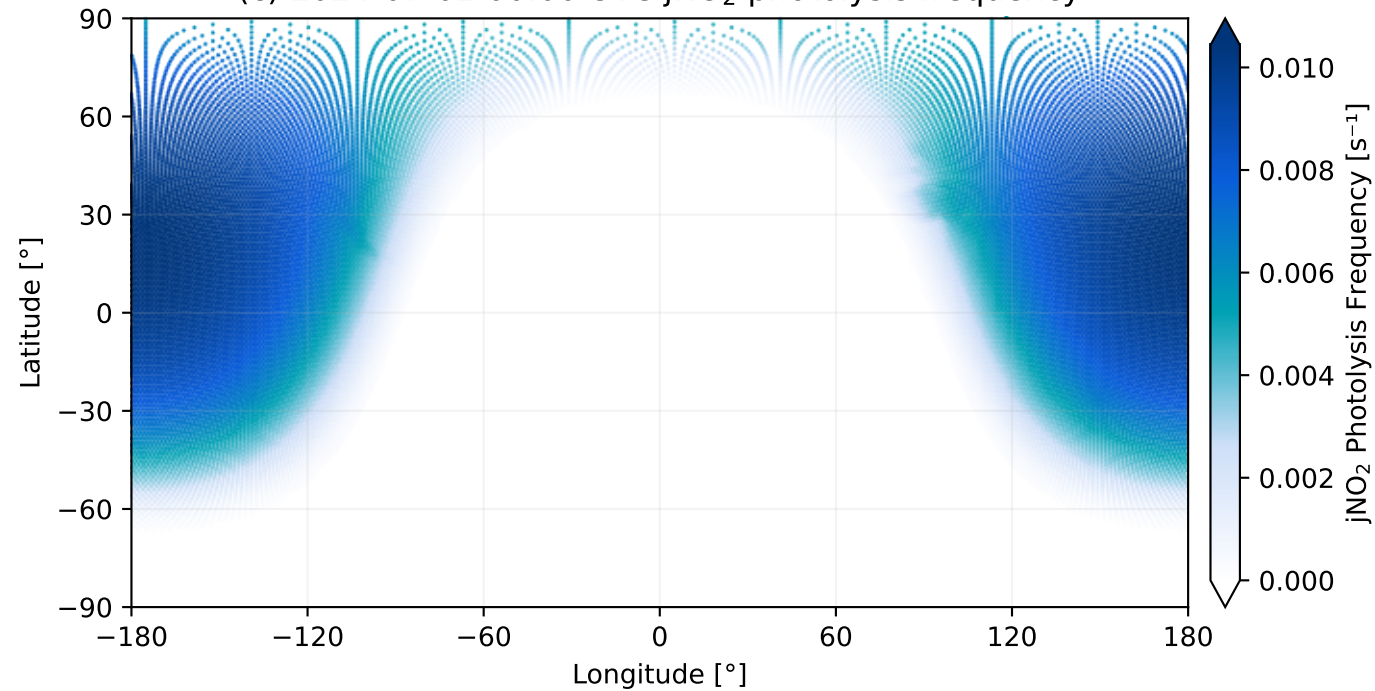
(c) 2024-07-02 00:00 UTC jNO 2 photolysis frequency
