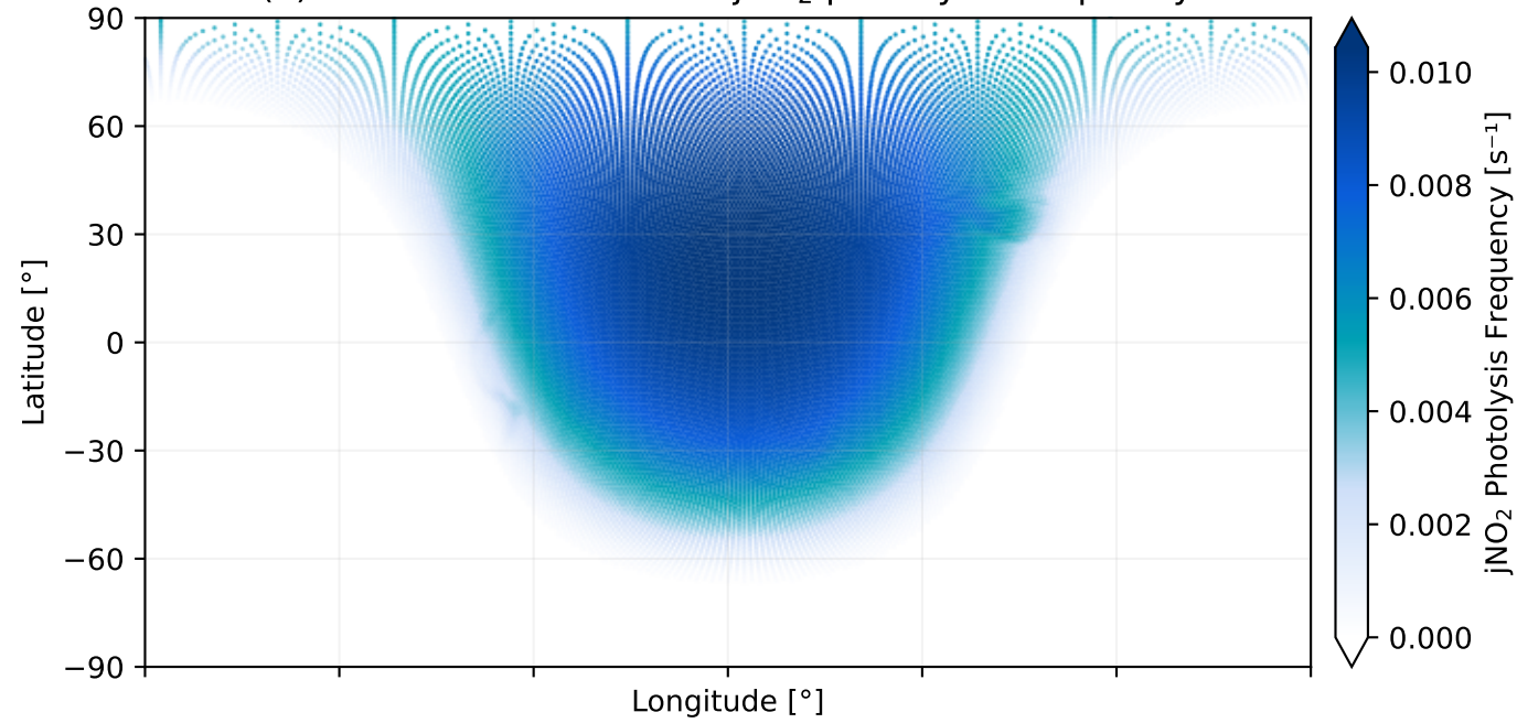
(c) 2024-07-02 00:00 UTC jNO 2 photolysis frequency
