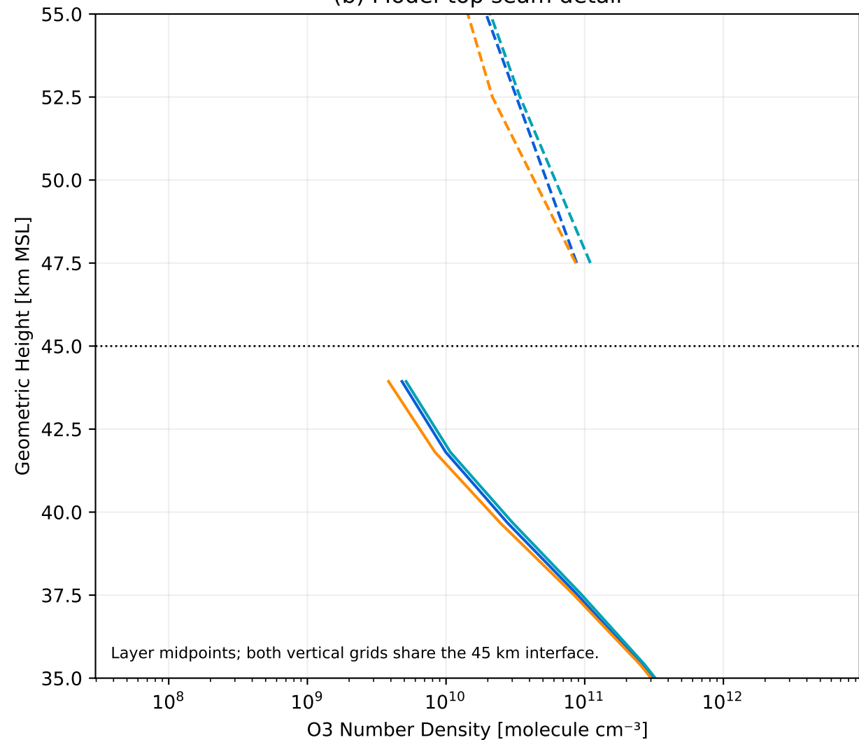
(b) Model-top seam detail
