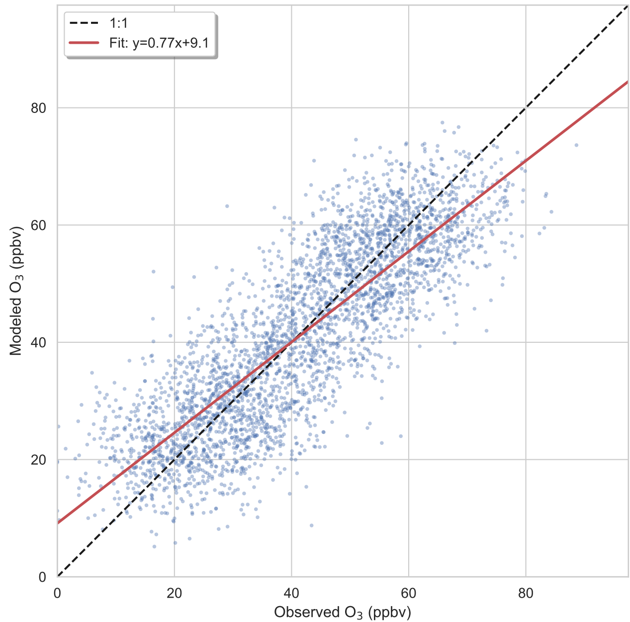
Scatter Plot
