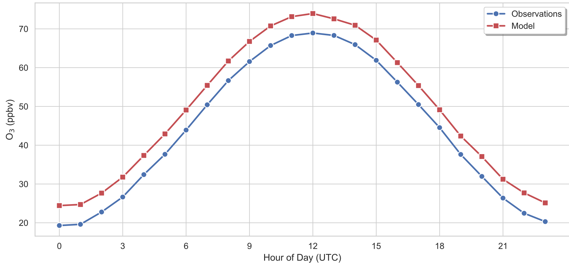
Diurnal Cycle of Ozone
