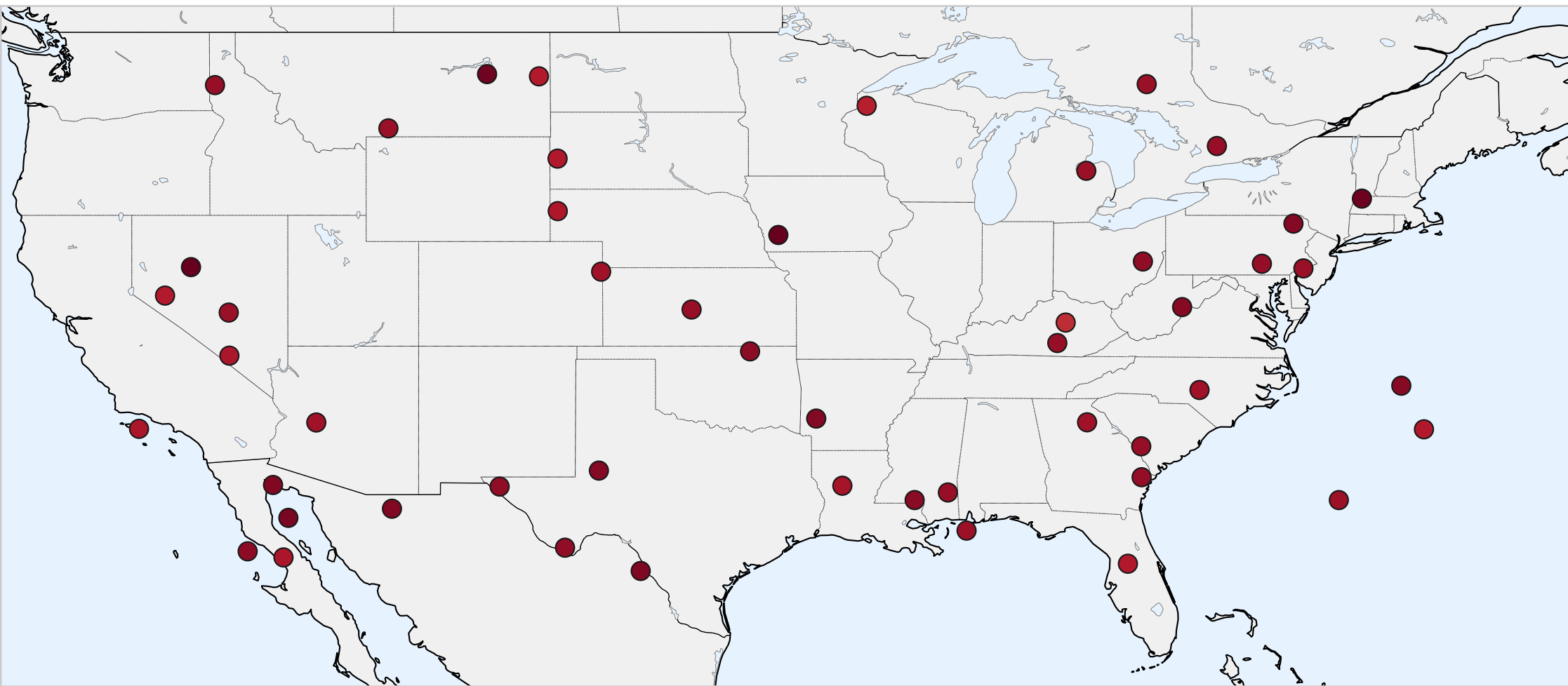
Mean O 3 Model Bias by Site
