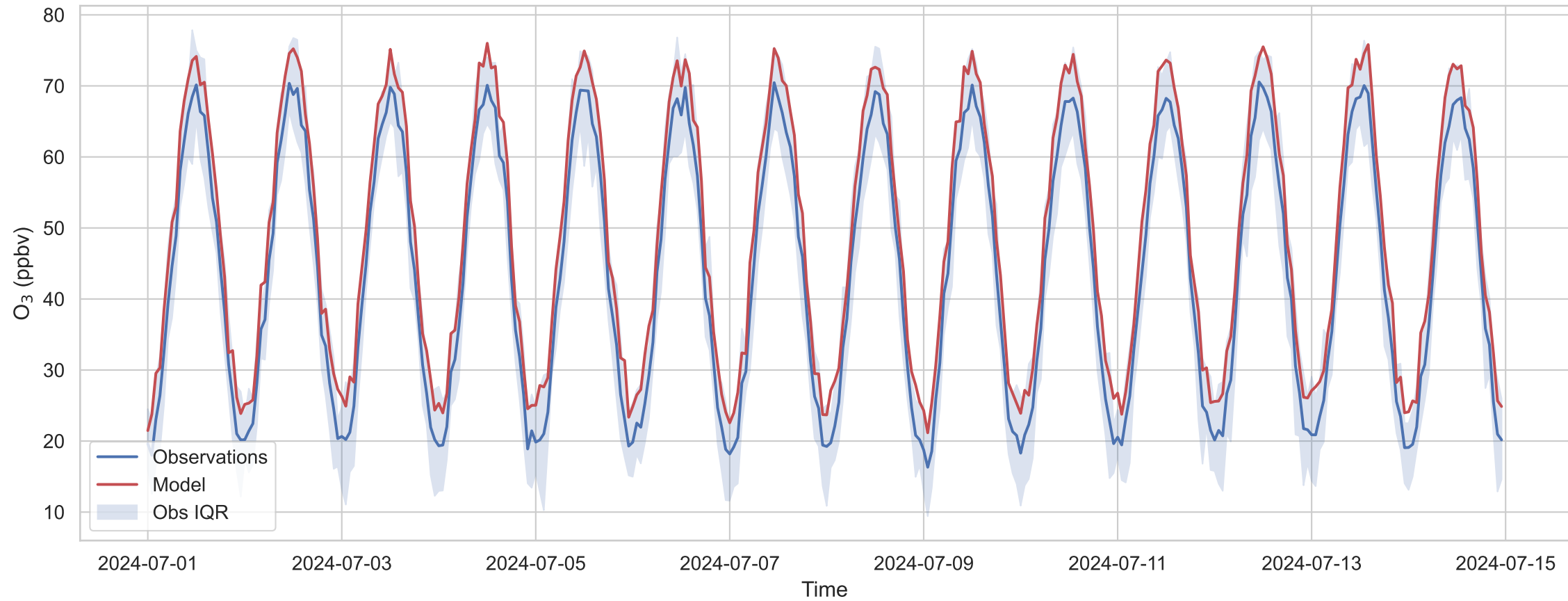
1. Time Series Plot
