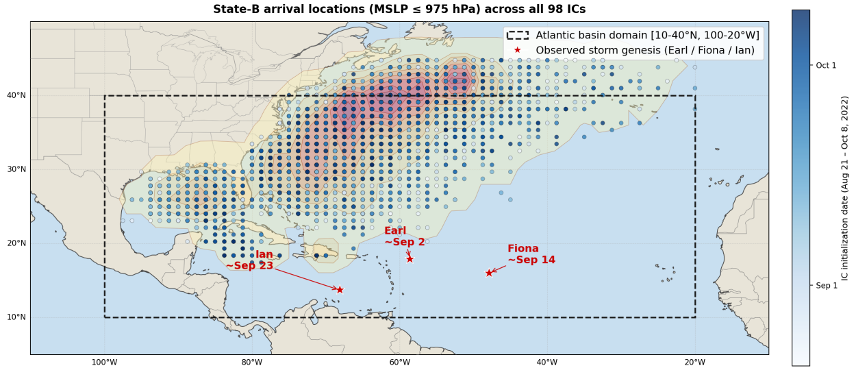
Figure 6: Geographic distribution of state- B arrival locations (MSLP \leq 975 hPa) across all 98 initial conditions. Each point marks where a reactive trajectory first reached state B ; colour encodes the IC initialisation date from August 21 (light) to October 8 (dark). The 2^\circ density contours (background) show the spatial clustering of genesis events across the season. Approximate observed genesis locations for Earl, Fiona, and Ian are annotated for reference. The distribution is concentrated in the tropical Atlantic, Caribbean, and Gulf of Mexico, consistent with observed 2022 Atlantic storm tracks, and shifts westward later in the season as Ian-like Gulf environments become active.
