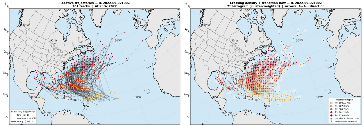
Figure 5: Reactive trajectories for the Hurricane Earl initial condition (2022-09-02T00Z), \sim 24 hours before genesis. Left : Spaghetti plot of FFS-generated reactive tracks (trajectories that ultimately reached state B , i.e., MSLP \leq 975 hPa). Track color indicates interface level; track weight encodes cluster size. Right : 2^\circ crossing-density histogram weighted by transition-flow, with arrows indicating the mean A \rightarrow B direction at each interface. The ensemble traces a tight recurving corridor northward along the US East Coast before spreading into the western North Atlantic, closely anticipating Earl’s observed track.
