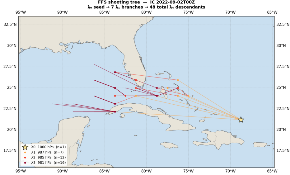
Figure 6: FFS shooting tree for the top geographically-spread \lambda_0 seed from the Earl IC (2022-09-02T00Z, config 0440_BN, rank 1 by \lambda_4 descendant count after applying a geographic-spread quality filter that excludes seeds whose descendants all cluster within a single grid cell). Points show the MSLP-minimum location at each 6-hour timestep, colored by interface level ( \lambda_0 = 1000 hPa through state B at 975 hPa). Branches fan northward from the genesis region, spanning a range of committed recurvature pathways along the US East Coast.
