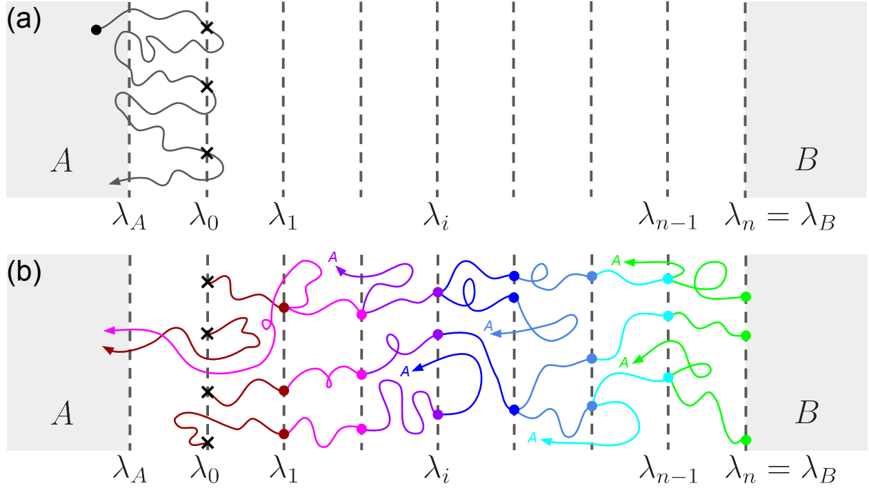
Figure 1: Schematic of the Forward Flux Sampling algorithm (after Allen et al. 2006). Panel (a), flux phase: Gray trajectories evolve forward from state A. Each decorrelated crossing of \lambda_0 is recorded (marked \times ). Panel (b), shooting phase: New trial trajectories are launched from each saved \lambda_i configuration (filled circles). Shots that return to state A (arrows labelled A) are failures; shots that reach \lambda_{i+1} (filled circles on the next interface) are successes, yielding the conditional probability P(\lambda_{i+1}|\lambda_i) . The genesis rate is k = \Phi_{A,0} \prod_i P(\lambda_{i+1}|\lambda_i) .
