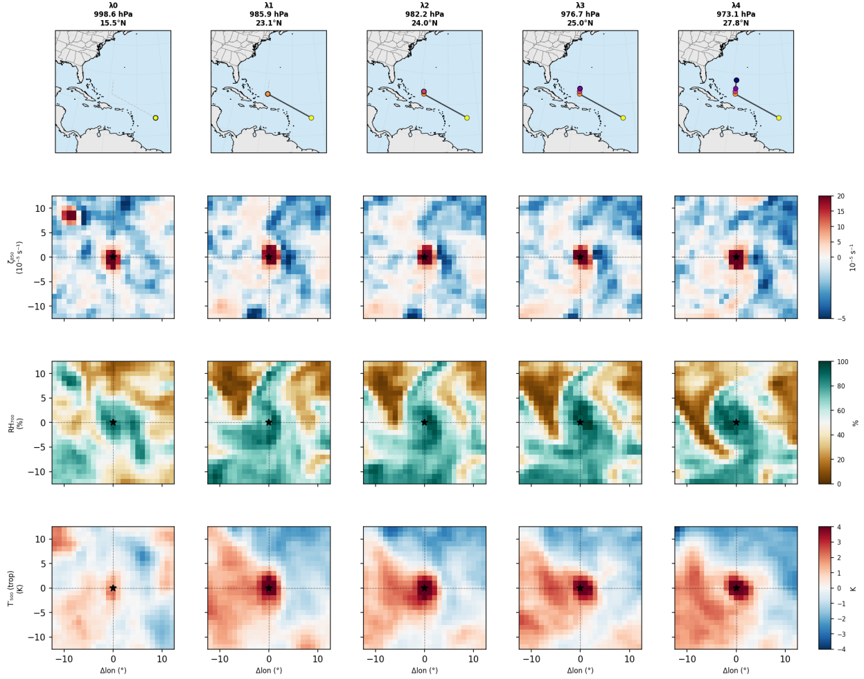
Figure 10: Storm-centred physics along a representative reactive pathway for the Earl IC (2022-09-02T00Z, pathway 1079), \lambda_0 through \lambda_4 . Each column shows one interface crossing. Column headers give the MSLP and storm latitude. The vortex originates near 16^\circ\text{N} in the eastern Atlantic at \lambda_0 and tracks west-northwestward to 28^\circ\text{N} at \lambda_4 , consistent with Earl’s observed tropical Atlantic genesis and subsequent westward motion. Row 1 : 850-hPa relative vorticity \zeta_{850} ( 10^{-5} \text{ s}^{-1} ). Row 2 : 700-hPa relative humidity \text{RH}_{700} (%). Row 3 : 500-hPa warm-core anomaly T'_{500} (K, relative to 0\text{--}30^\circ\text{N} mean). The persistent cyclonic vorticity and warm-core anomaly at each interface confirm continuous vortex identity and warm-core structure through state B . Pathways where the warm core collapses at high latitudes are screened out by the CPS filter and not included in the genesis rate calculation.
