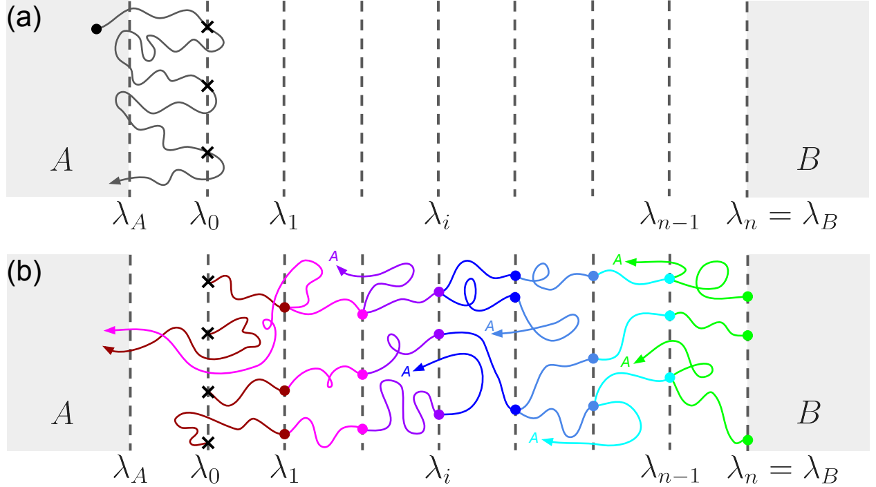
Figure 1: Schematic of the Forward Flux Sampling algorithm (after ?). Panel (a) — flux phase: Gray trajectories evolve forward from state A; each decorrelated crossing of \lambda_0 is recorded (marked \times ). Panel (b) — shooting phase: New trial trajectories are launched from each saved \lambda_i configuration (filled circles). Shots that return to state A (arrows labelled A) are failures; shots that reach \lambda_{i+1} (filled circles on the next interface) are successes, yielding the conditional probability P(\lambda_{i+1}|\lambda_i) . The genesis rate is k = \Phi_{A,0} \prod_i P(\lambda_{i+1}|\lambda_i) .
