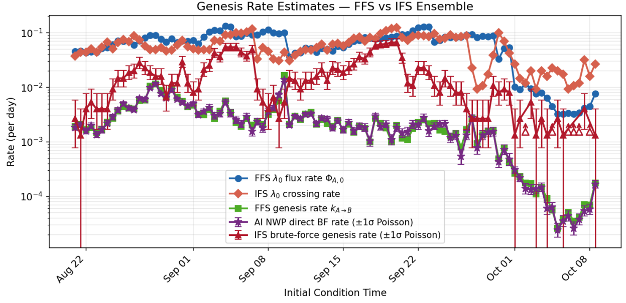
Figure 2: FFS genesis rates across all 98 initial conditions (August 21 – October 8, 2022) on a logarithmic scale. Blue : \lambda_0 flux rate \Phi_{A,0} . Orange : IFS \lambda_0 crossing rate (contextual reference; not directly comparable to FFS due to different resolution and no CPS filter). Green : Full FFS genesis rate k^{\text{FFS}} (flux \times product of conditional probabilities). Purple : Direct-sampling rate k^{\text{direct}} from state- B arrivals during the flux phase ( \pm 1\sigma Poisson). Red : IFS brute-force genesis rate ( \pm 1\sigma Poisson; upward arrows denote upper bounds where zero events observed). Agreement between green and purple (mean ratio 1.03 \pm 0.15 ) validates the FFS method. The FFS rate resolves a seasonal cycle spanning nearly three orders of magnitude invisible to direct 50-member ensemble sampling.
