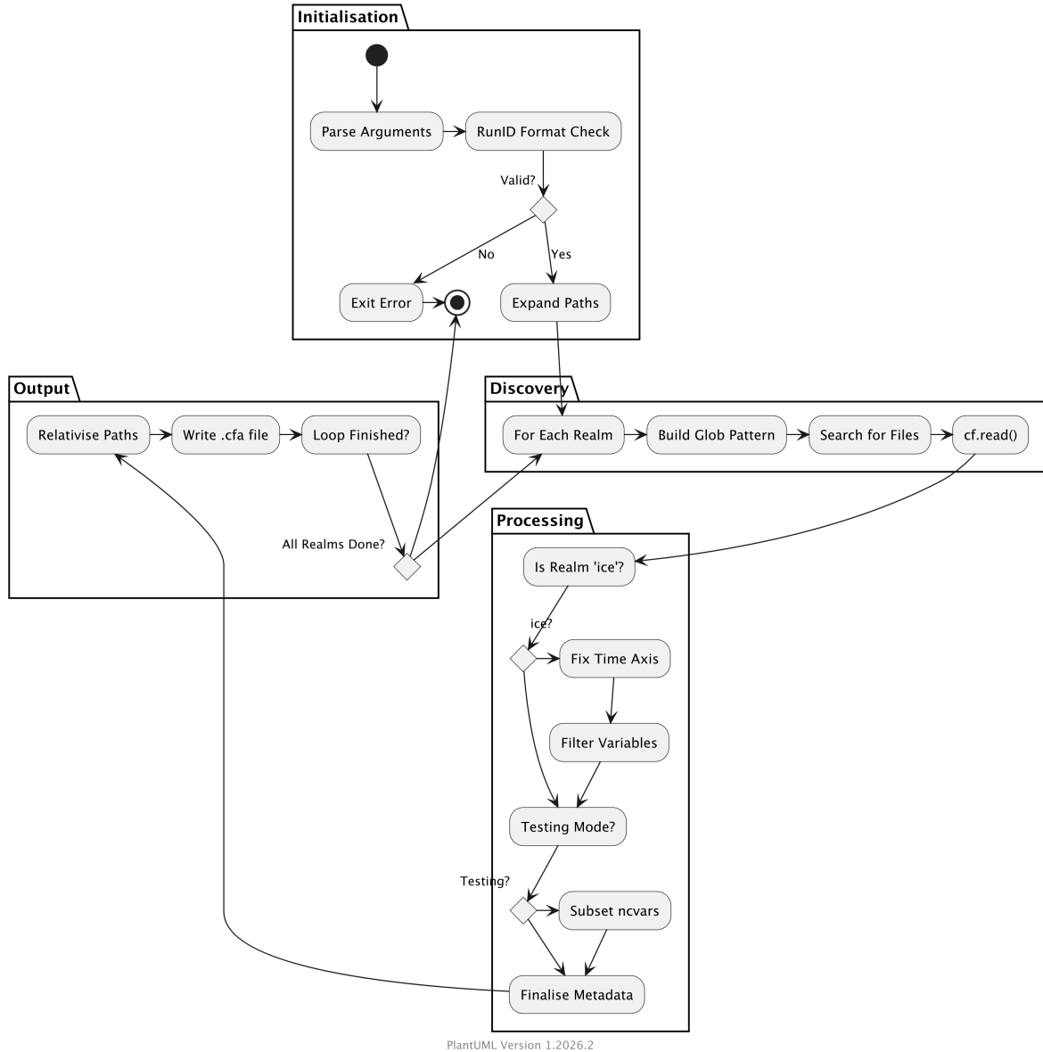
Figure 4: Algorithm for the seed.py file, prepared with PlantUML [Roques, 2026].
