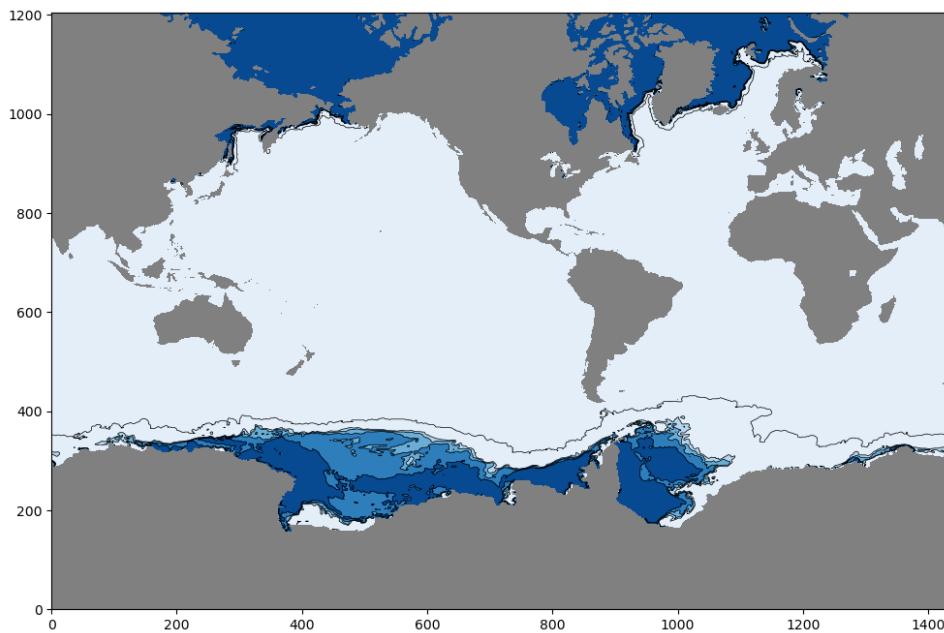
Figure 15: Example sea ice area from ensemble member 1 of the historical ensemble.
