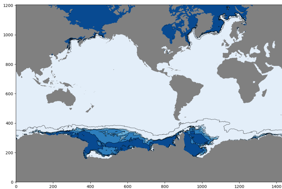
Figure 16: Example sea ice area (aggregate) from ensemble member 1 of the historical ensemble. The quantity is dimensionless and the contour lines shown are at 0 (no ice), 0.2, 0.4, 0.6, 0.8 and 1 (full coverage).
