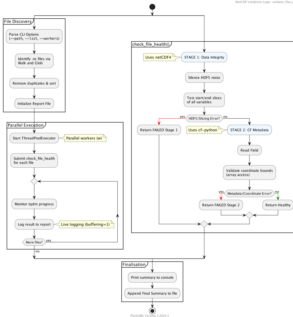
Figure 19: Algorithm for the validate-files.py file, Figure prepared using PlantUML.
