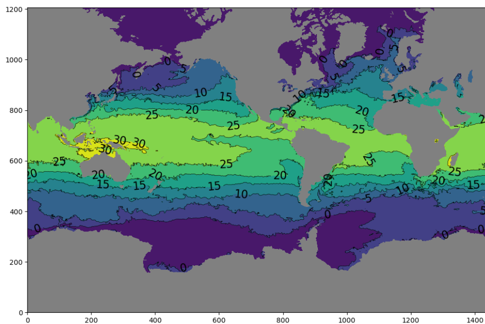
Figure 15: Example sea surface temperature (in Celsius) from ensemble member 1 of the historical ensemble.
