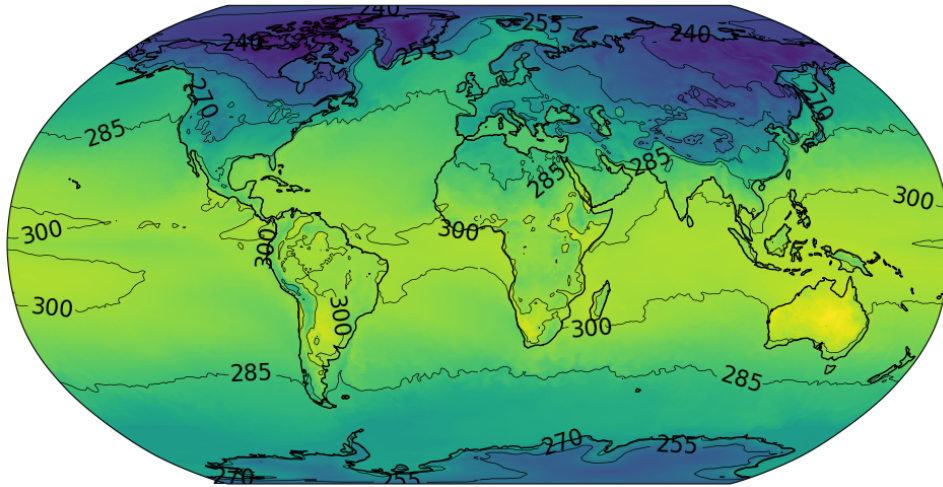
Figure 14: Example surface temperature after timestep (in Kelvin) from ensemble member 1 of the historical ensemble.
