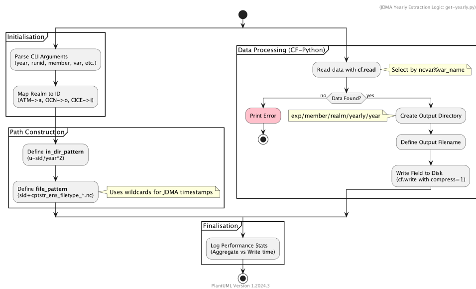
Figure 18: Algorithm for the get-yearly.py file, Figure prepared using PlantUML.
