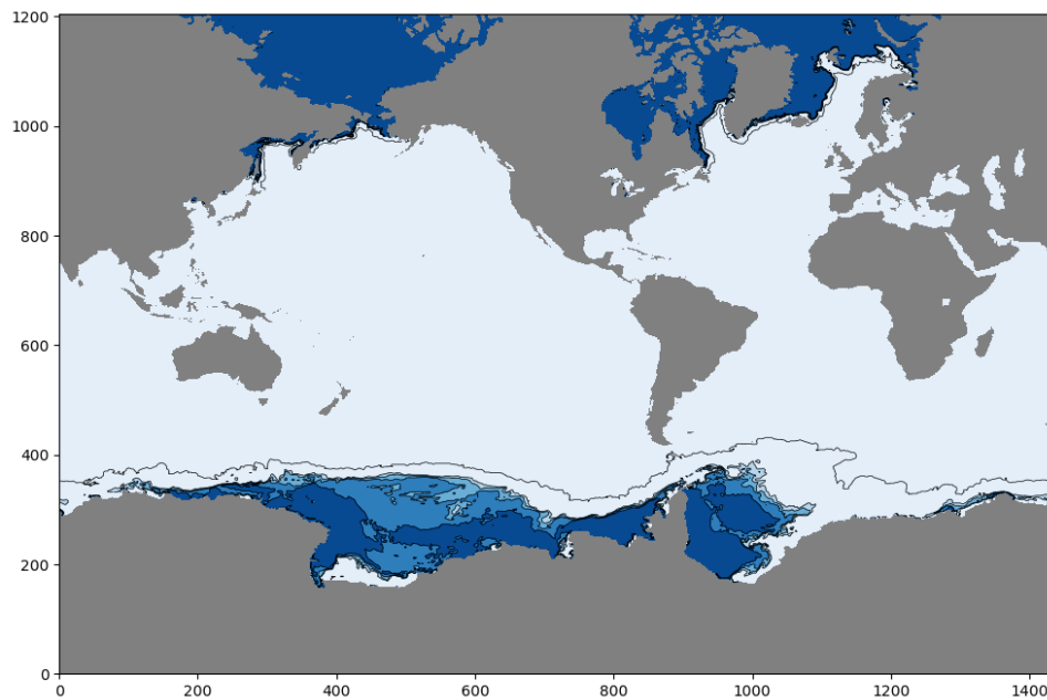
Figure 15: Example sea ice area (aggregate) from ensemble member 1 of the historical ensemble. The quantity is dimensionless and the contour lines shown are at 0 (no ice), 0.2, 0.4, 0.6, 0.8 and 1 (full coverage).
