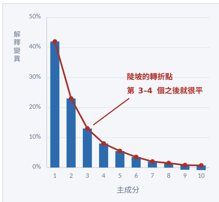
左・陡坡圖 Scree Plot
