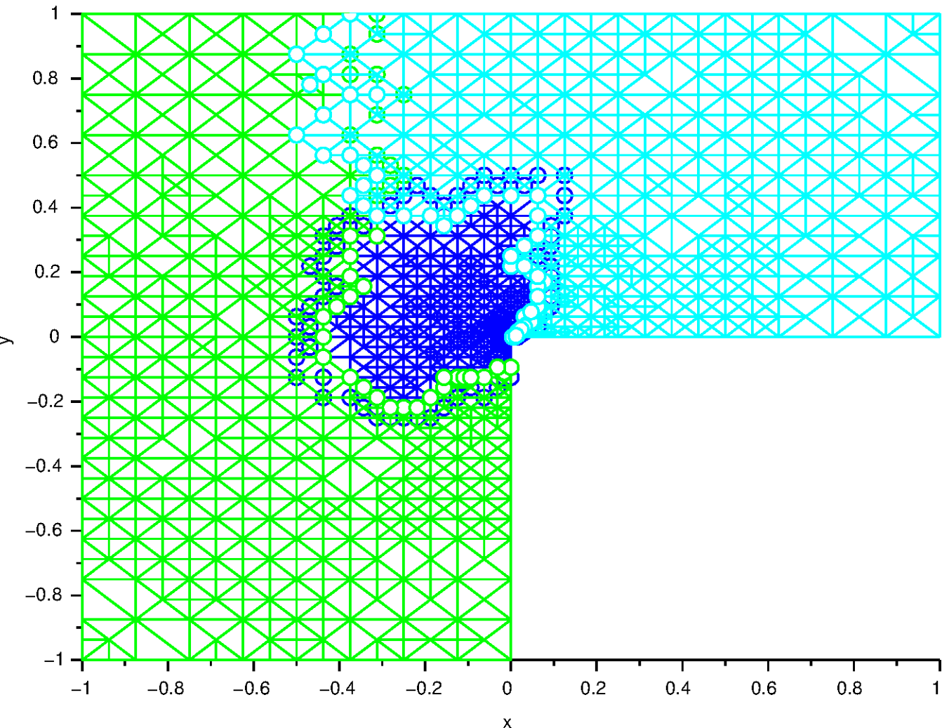
L domain
