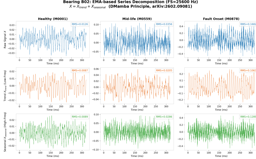
Figure 3: Waveform decomposition results on bearing B02 across three representative phases: healthy, mid-life, and fault onset.
