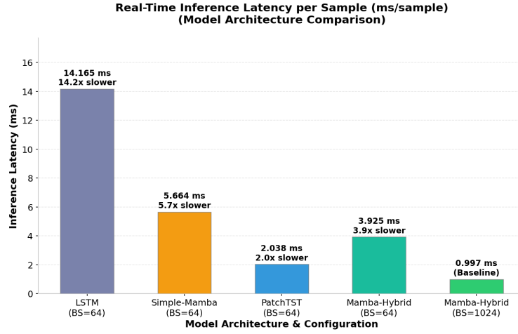
Figure 4: Real-time model inference latency comparison per sample (ms/sample) across different model architectures and batch size (BS) configurations. Under the massive parallel throughput workload ( BS = 1024 ), a baseline inference latency of 0.997 ms per sample is achieved by the proposed Mamba-Hybrid model. In contrast, substantial slowdowns are exhibited by the other tested architectures: PatchTST ( BS = 64 ) is 2.0 \times slower, Mamba-Hybrid ( BS = 64 ) is 3.9 \times slower, Simple-Mamba ( BS = 64 ) is 5.7 \times slower, and LSTM ( BS = 64 ) is 14.2 \times slower. Slowdown ratios are annotated directly above each corresponding bar relative to the high-throughput Mamba-Hybrid baseline.
