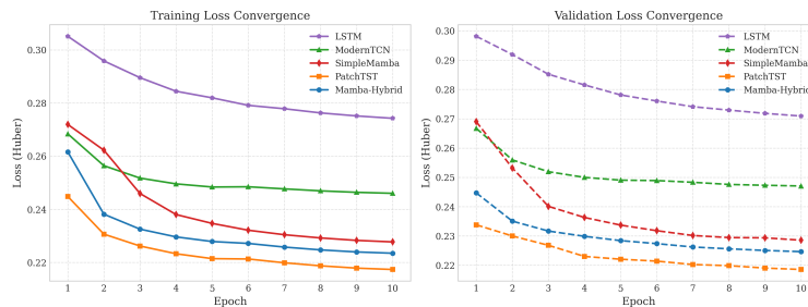
Figure 2: Training and validation Huber loss convergence curves across 10 training epochs for all benchmarked architectures under parameter budget parity.
