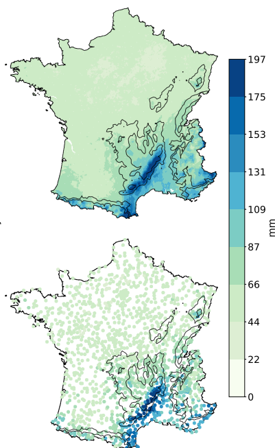
10-year return level of daily precipitation
