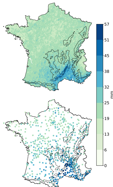
10-year return level of hourly precipitation
