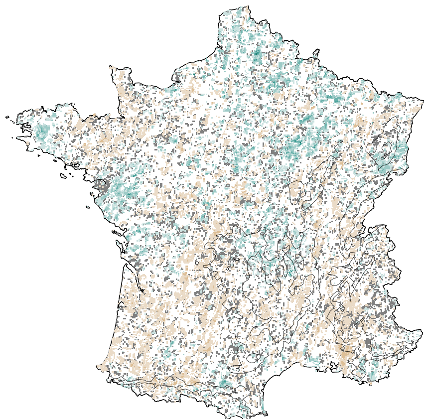
AROME
