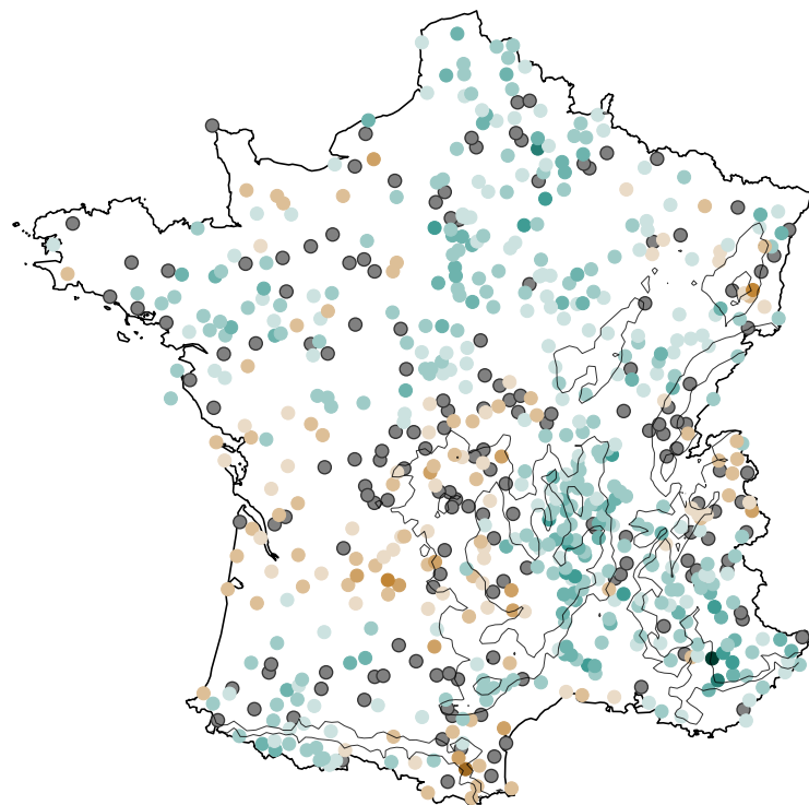
(b) Stations — Daily RL_2 trend
