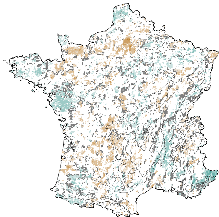
(a) AROME — Daily RL_2 trend
