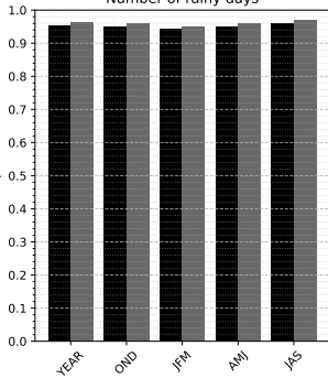
Number of rainy days
