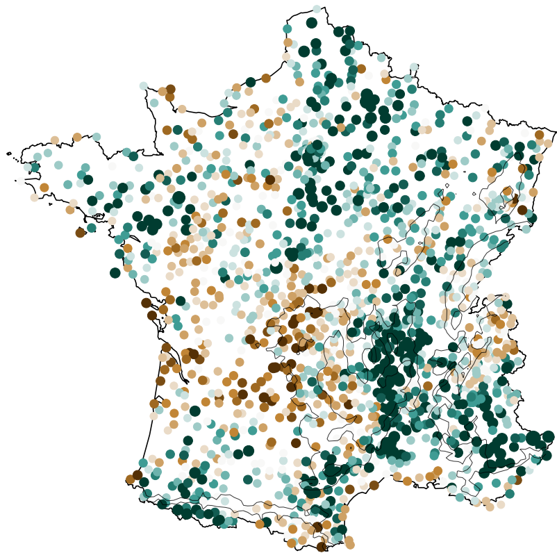
(a) Observed Annual Maxima Trend (%)
