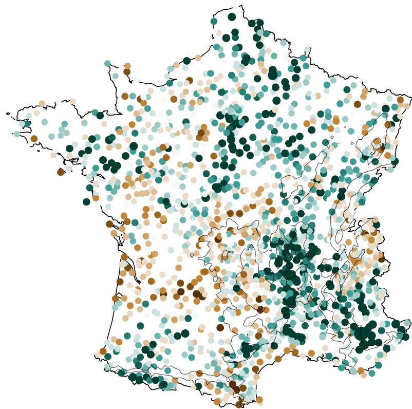
(b) GEV RL_2 Trend (%)
