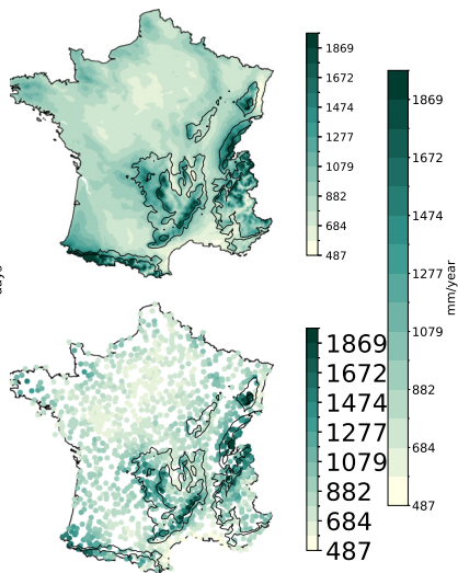
Annual total precipitation
