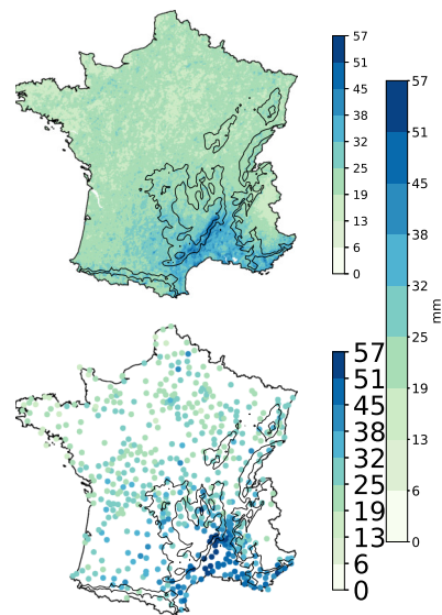
10-year return level of hourly precipitation
