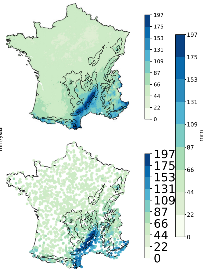
10-year return level of daily precipitation
