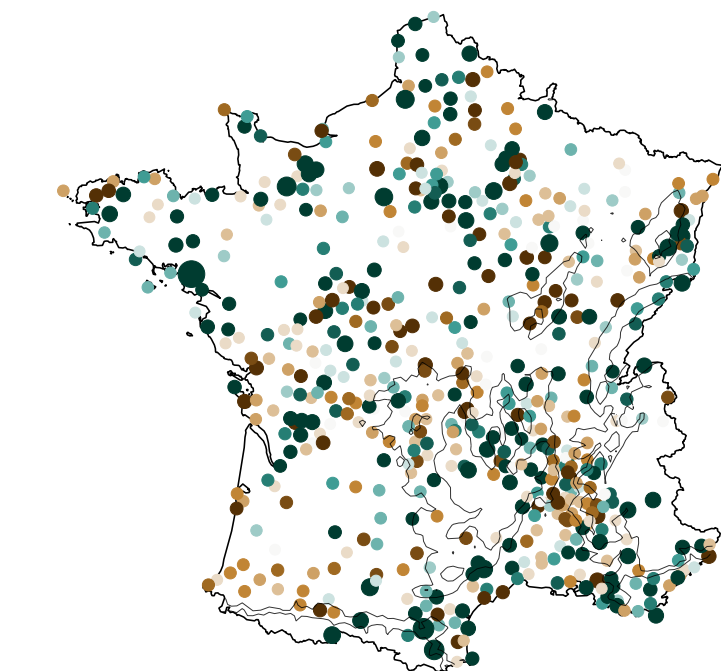
(a) Observed Annual Maxima Trend (% , Hourly)
