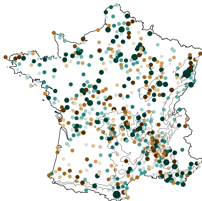
(b) GEV Mean Trend (% , Hourly)
