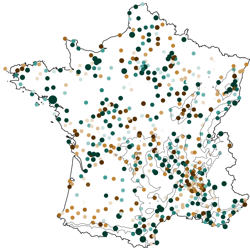
(a) Observed Annual Maxima Trend (% , Hourly)
