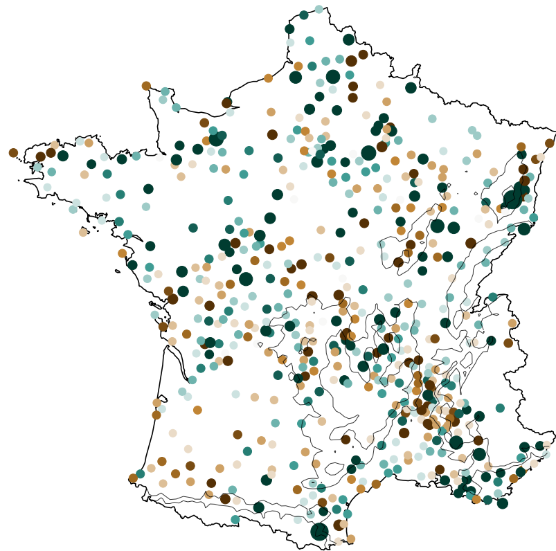
(b) GEV Mean Trend (% , Hourly)
