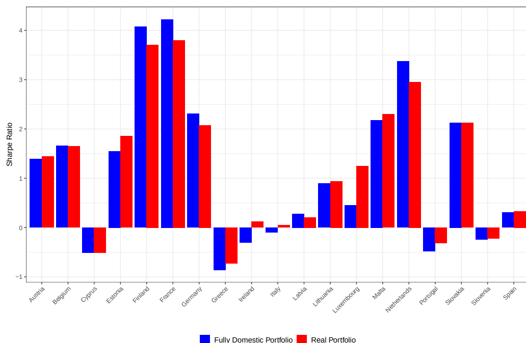
Figure 66: Sharpe Ratios Comparison (2010–2021). The figure compares Sharpe ratios across euro area countries, computed using the 1-month Euribor as the risk-free rate and ESCB equity returns.
