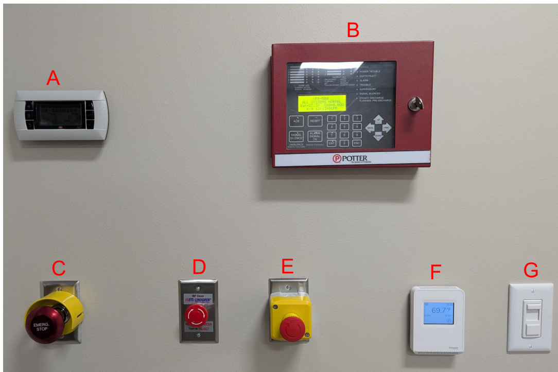
Figure 2: Control Room button wall. A Haskris Coolant Sounder. B Fire System Board. C Emergency Power Off. D Magnet Door release. E Fire suppression trigger. F Thermostat. G Light switch.
