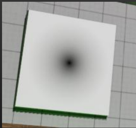
BP_BrakableWall
