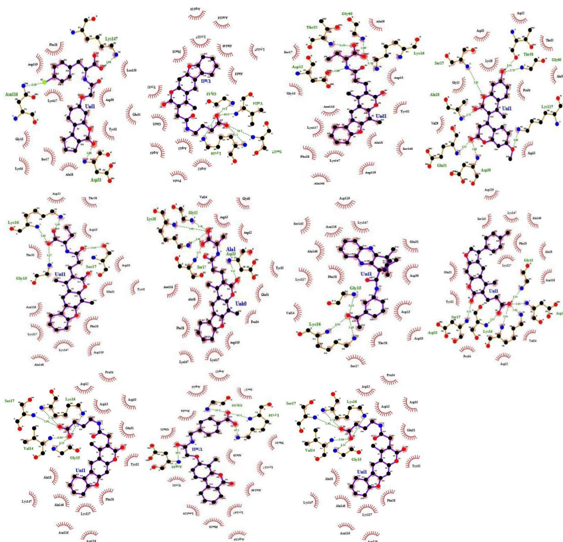
Figure 2. Comparative 2D representations of protein-ligand interactions for docked complexes, generated using LigPlot+.
