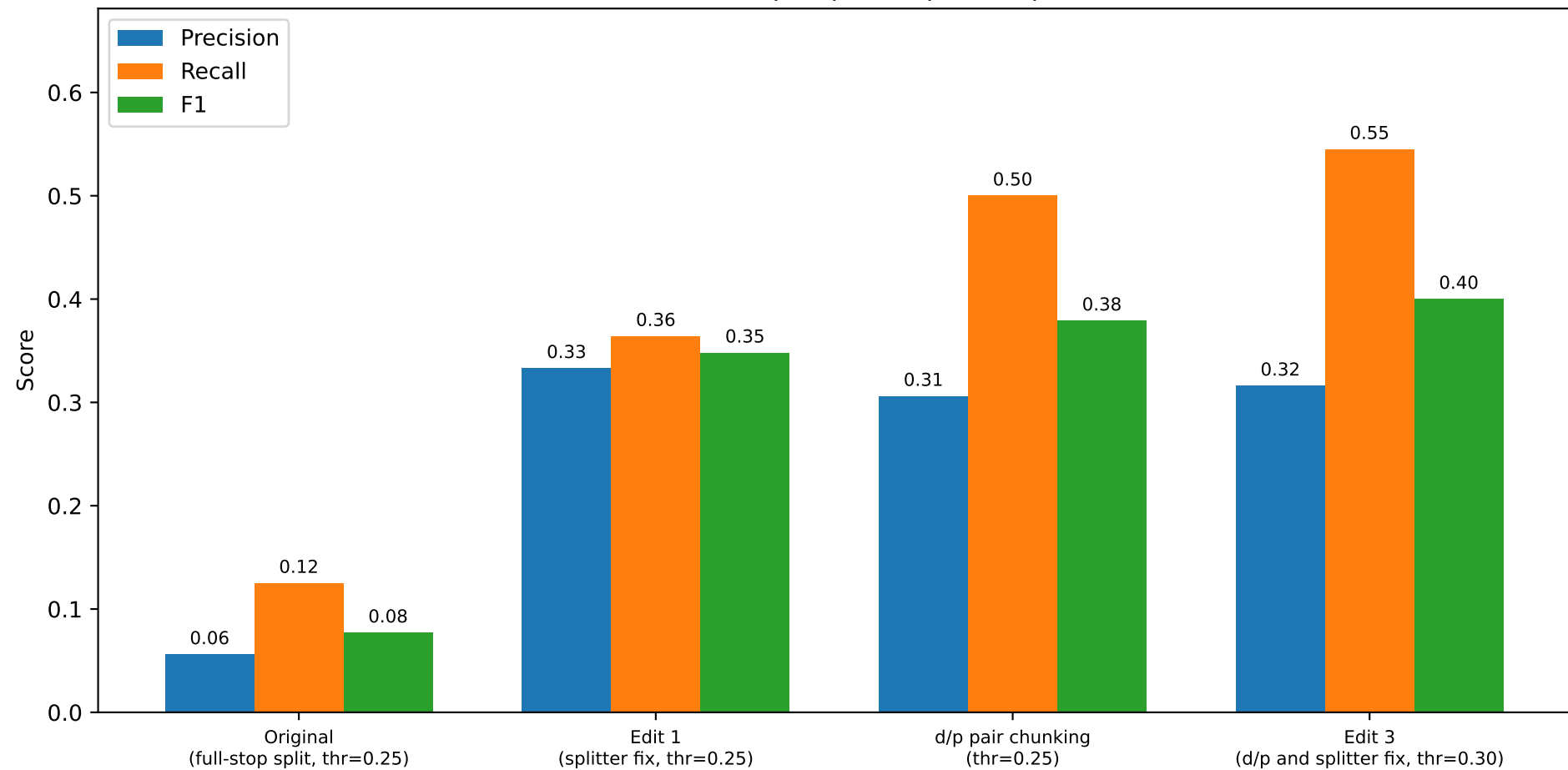
Figure: AlignScoreChecker hallucination-direction P/R/F1 across each edit (same 10-file sample: prim1, prim10-prim18)
