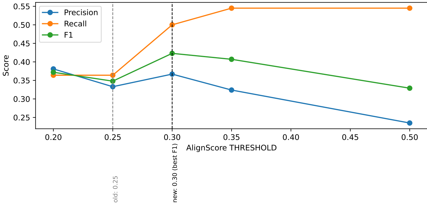
Figure: threshold re-sweep after the splitter fix (Edit 1 + Edit 3) hallucination labels only, 10-file sample, scores cached from one model pass
