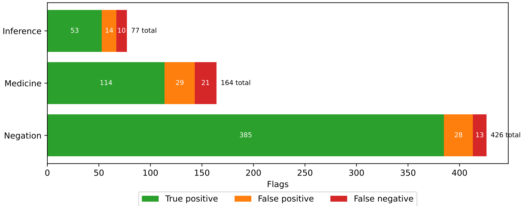
Figure 11: TP / FP / FN by extraction type (57 files)
