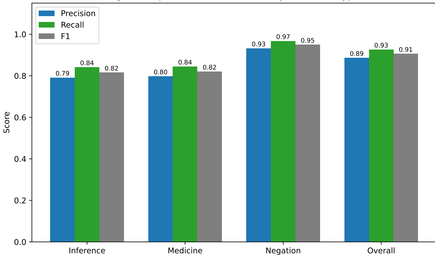
Figure 12: precision, recall, and F1 by extraction type
