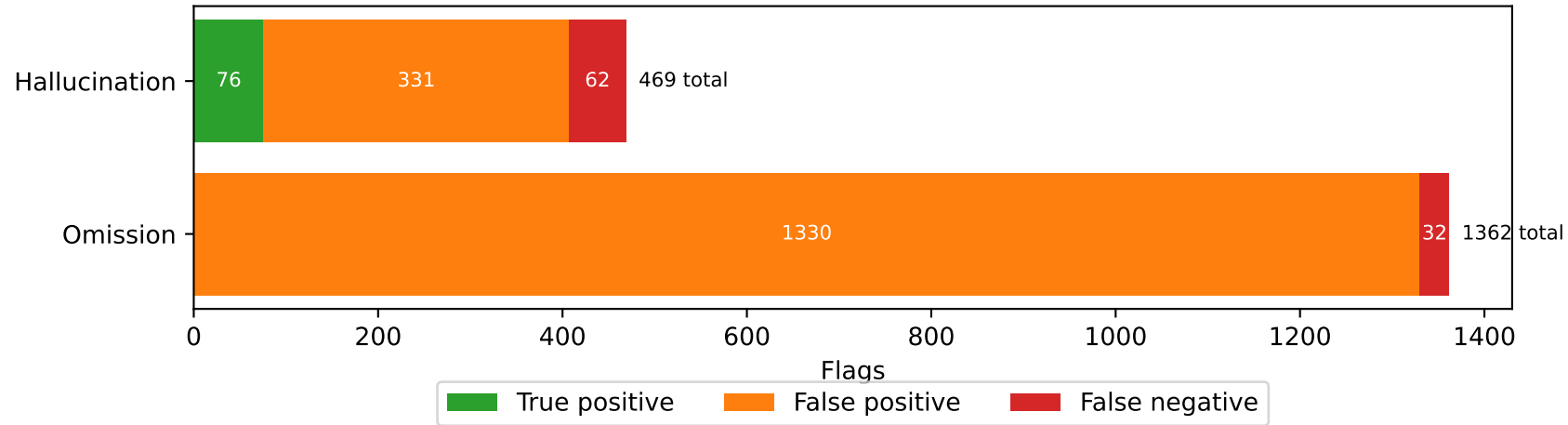
Figure: EmbedKDECheck TP / FP / FN by direction (57 files)
