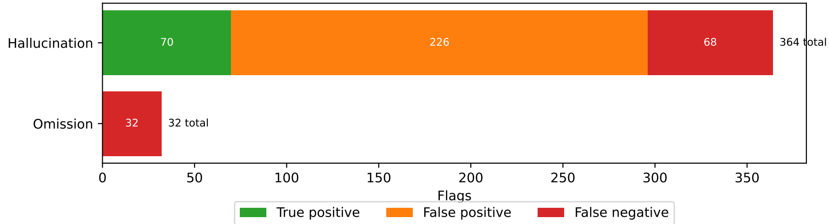
Figure: AlignScore TP / FP / FN by direction (57 files)
