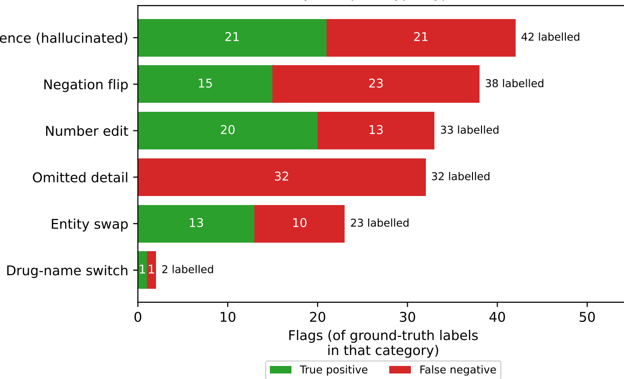
By corruption type (typed)
