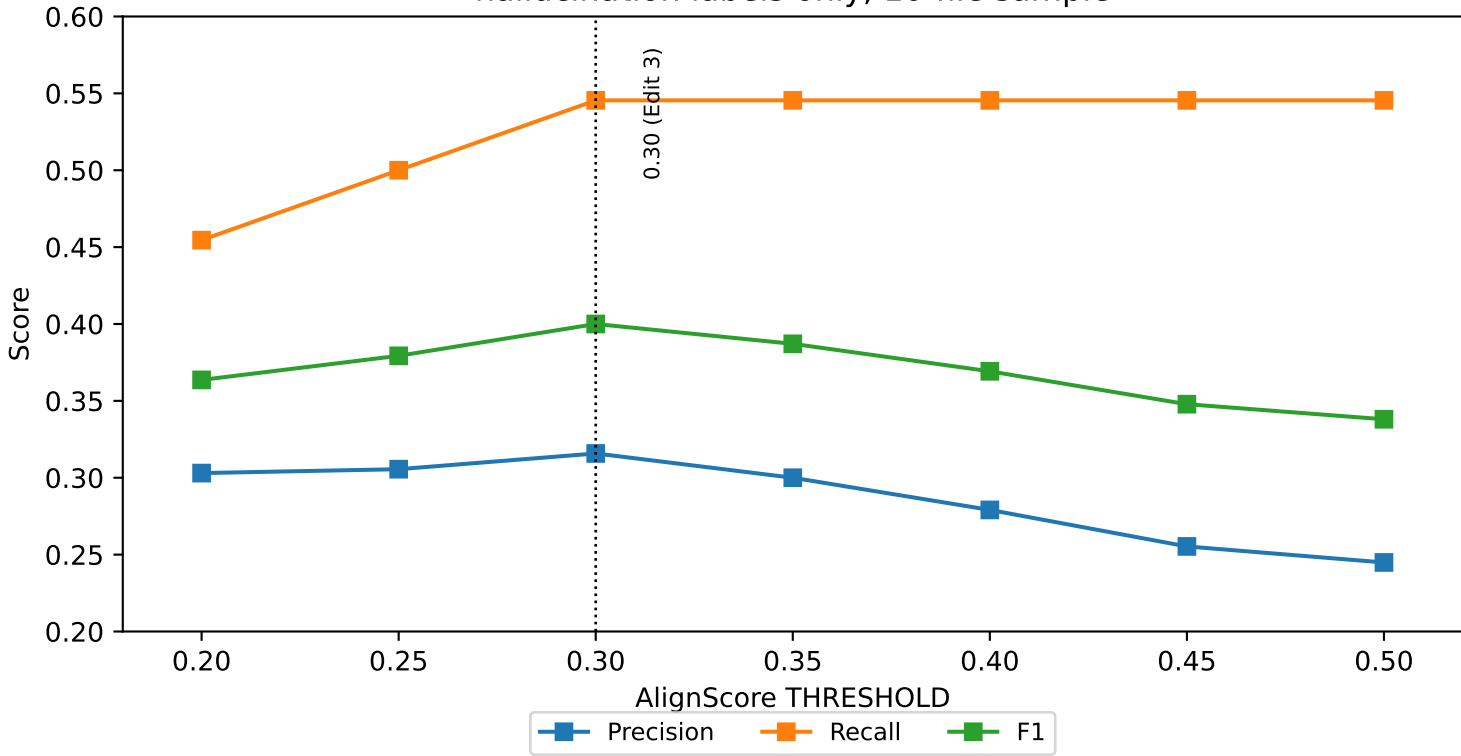
Figure: d/p pair chunking Precision/Recall/F1 vs threshold from 0.20, hallucination labels only, 10-file sample
