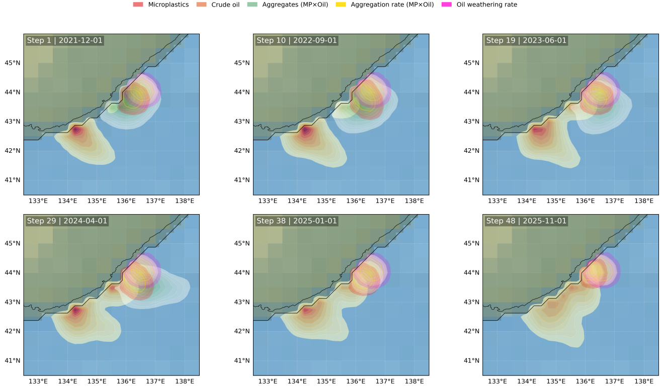
Figure 2: Six sampled times from the dataset-driven surface multispecies proxy. The overlays show normalized microplastic, crude-oil, and aggregate fields together with aggregation and oil-weathering rates. The land mask blocks the proxy fields. Because each species is normalized independently after every substep, this panel is qualitative evidence of transport and reaction structure rather than a mass forecast.
