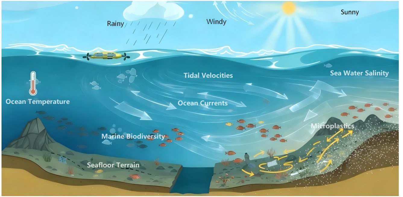
Figure 1: Conceptual view of the environmental channels and ecological signals represented by, or targeted for coupling with, OneOcean. It illustrates terrain, currents, tidal velocity, thermohaline variables, weather, biodiversity, and microplastics; it is not a scale diagram and does not imply that every release variant contains every depicted field.
