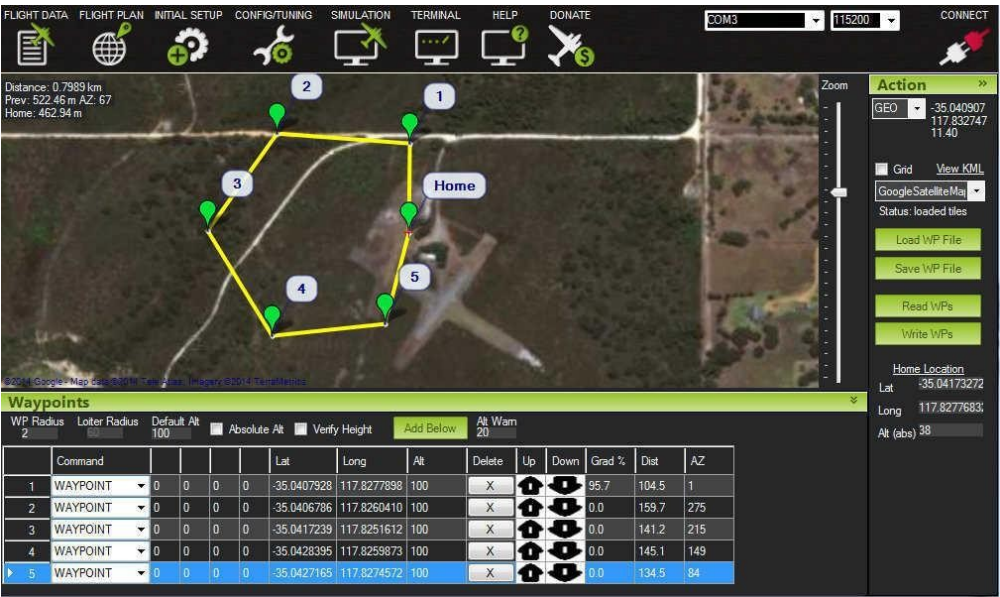
Figure 3.10: Mission Planner Autonomous Waypoint Mission Plan
