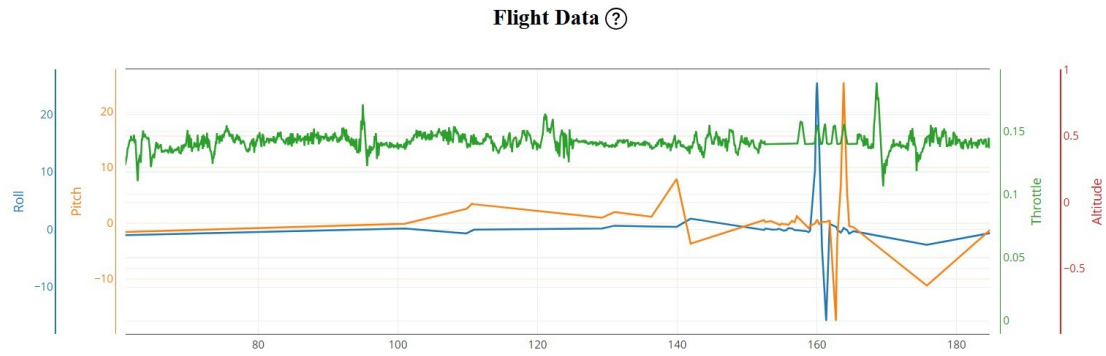
Figure 4.22: Flight Data Log: Roll, Pitch and Throttle against Time
