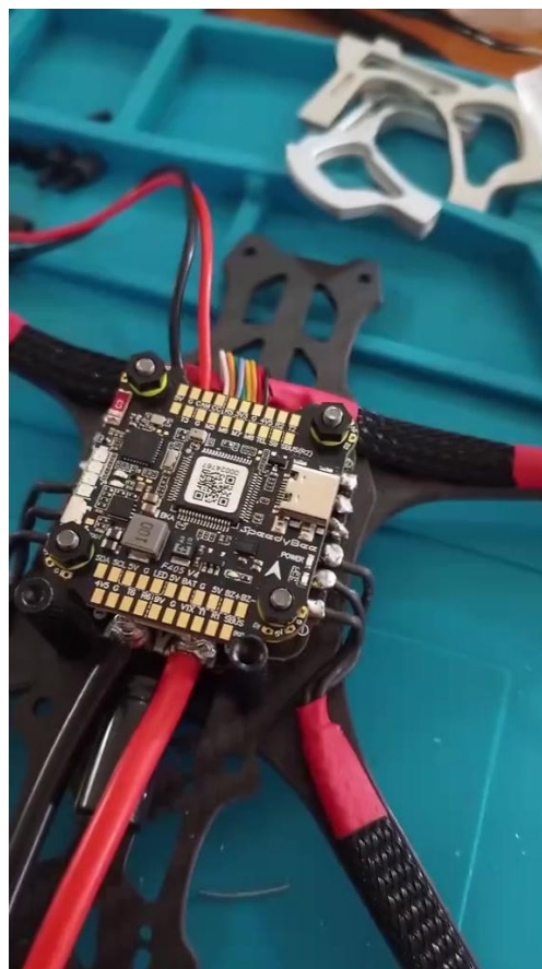
Figure 3.5: Flight Controller Stack Assembly
