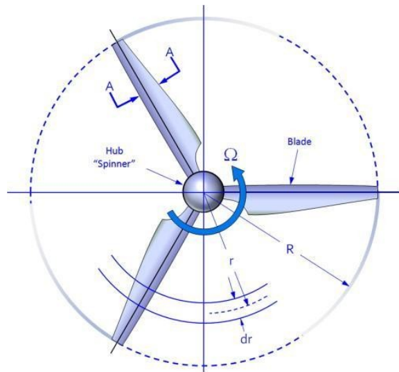
Figure 2.7: Tri-blade Propeller Aerodynamic Profile and Blade Element Diagram
