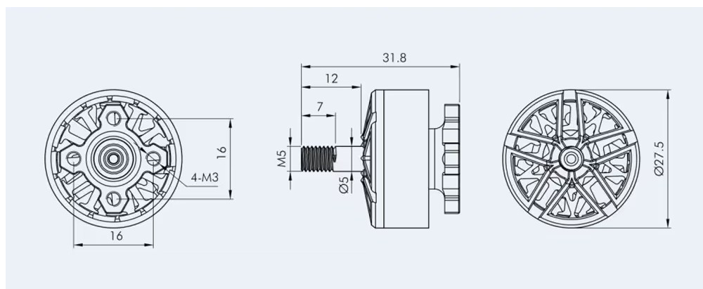
Figure 2.6: T-Motor Velox V2207 V3 Motor Dimensional Drawing (dimensions in mm)
