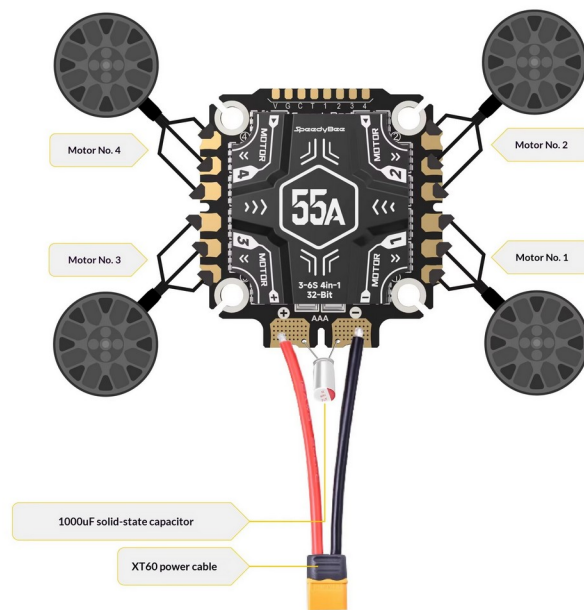
Figure 3.4: ESC–Motor and Power Wiring Diagram (M1–M4 ESC outputs correspond to the four motor positions)
