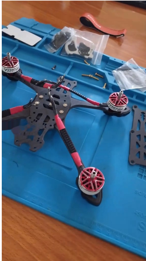
Figure 3.3: Motor Mounting and Propeller Installation
