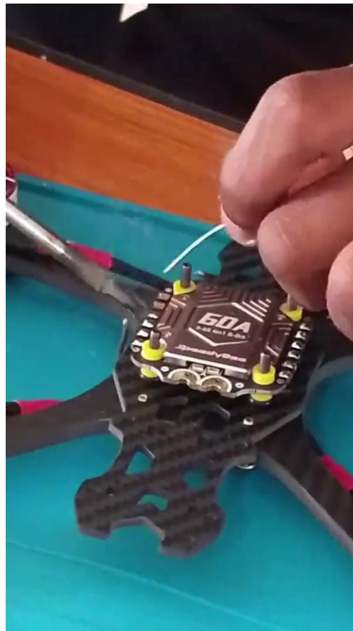
Figure 2.4: SpeedyBee 4-in-1 ESC Being Installed on the Frame
