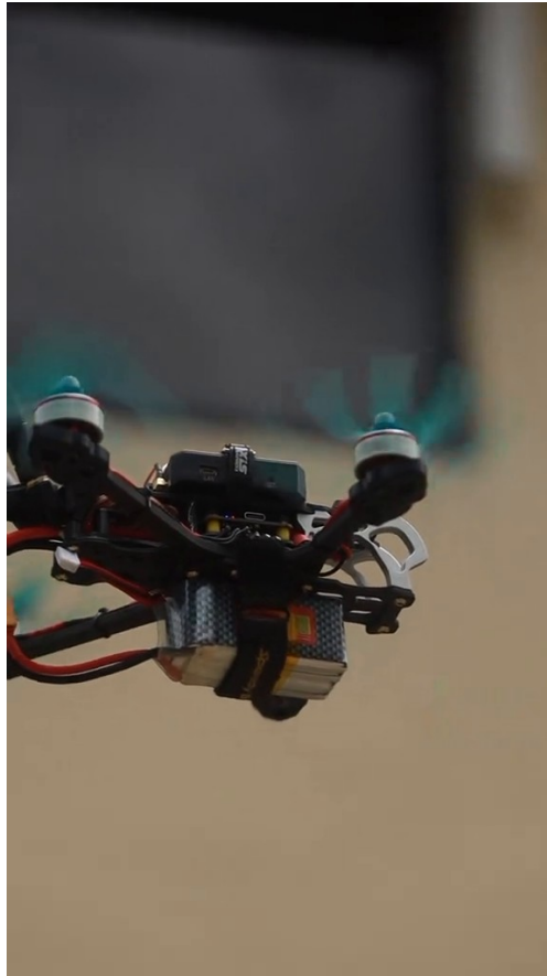
Figure 3.12: Completed Drone Assembly: Side View in Flight
