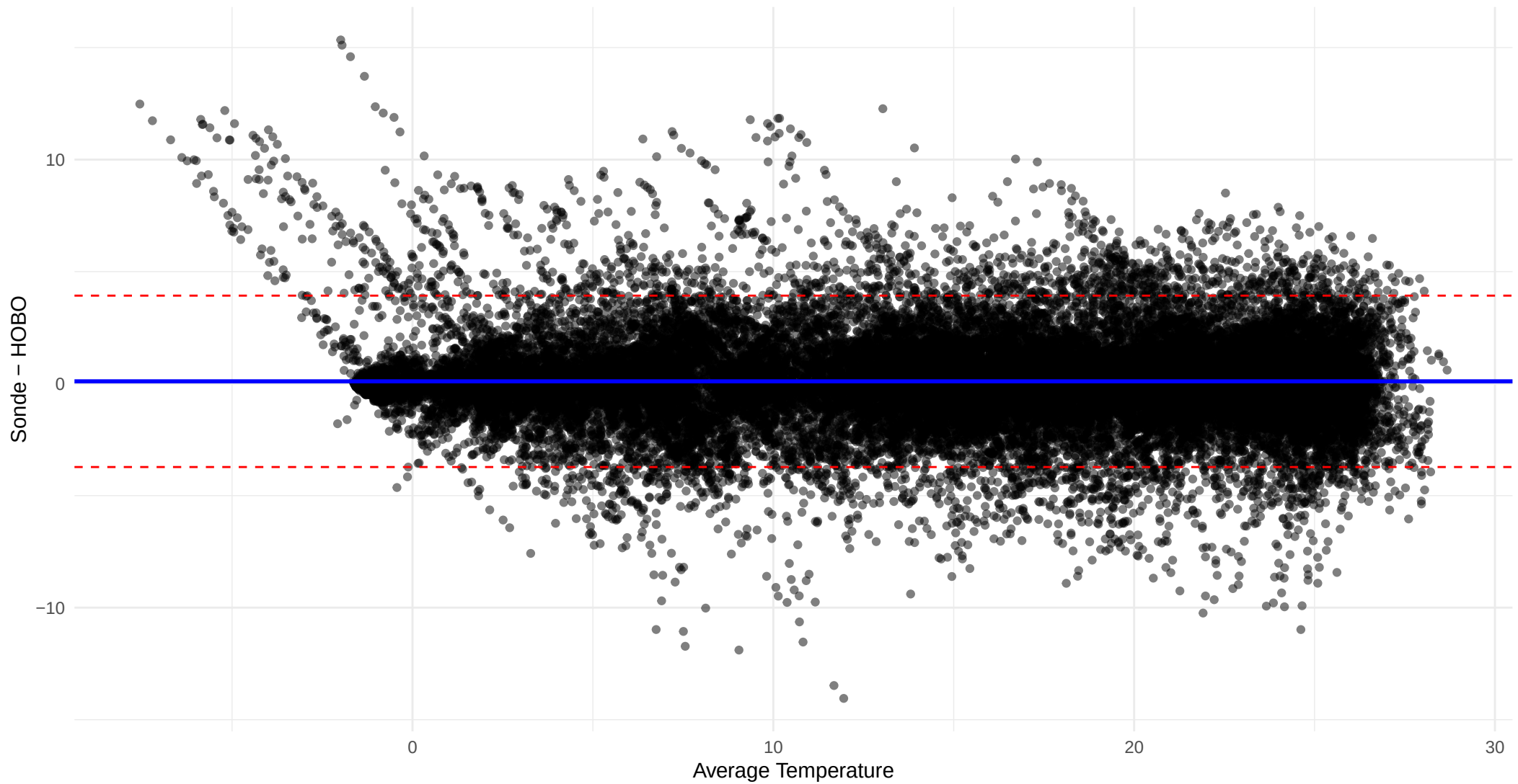
Ash Creek Bland-Altman Agreement Plot
