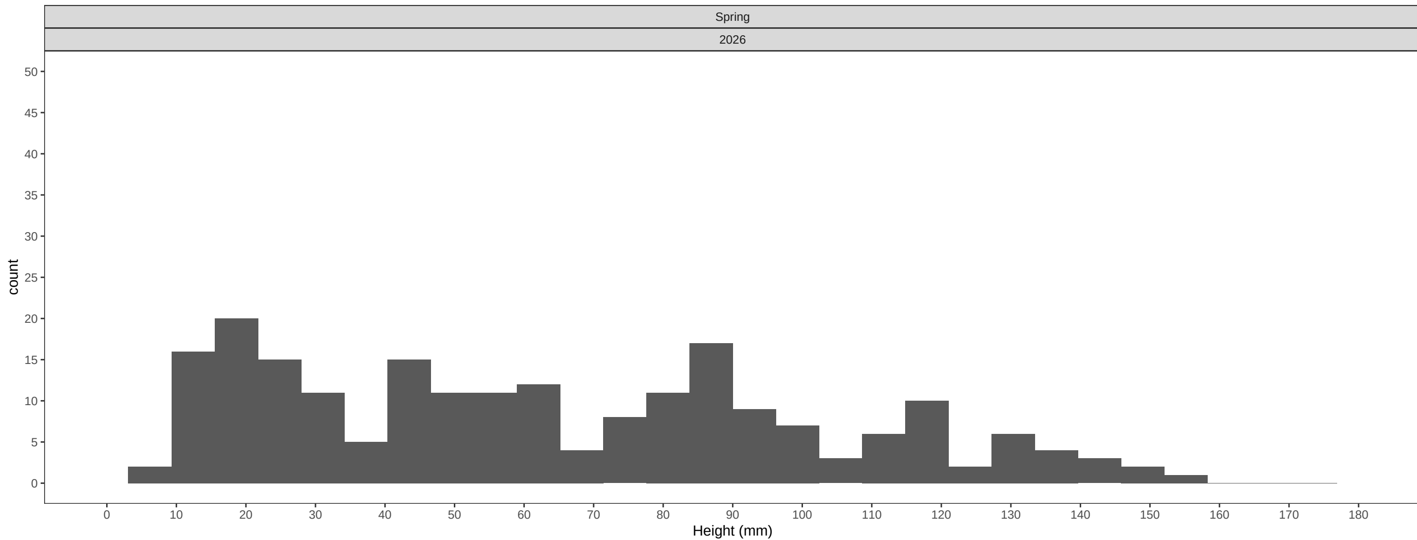
Fence Creek Height Dead Oysters
