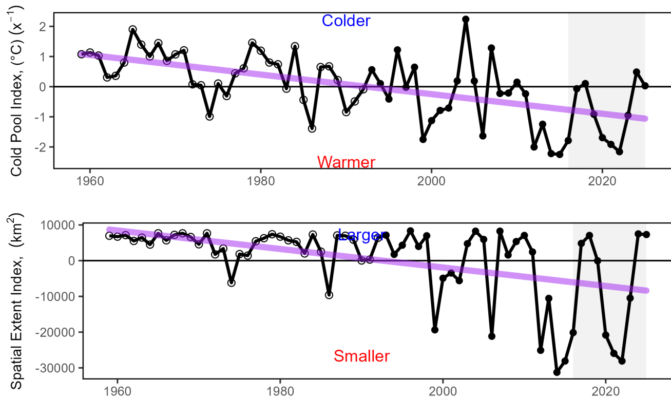
Figure 46: Seasonal cold pool mean temperature (top) and spatial extent index (bottom), based on bias-corrected Regional Ocean Modeling System-Northwest Atlantic (ROMS-NWA) (open circles) and GLORYS (closed circles), with long-term declining trends (purple).
