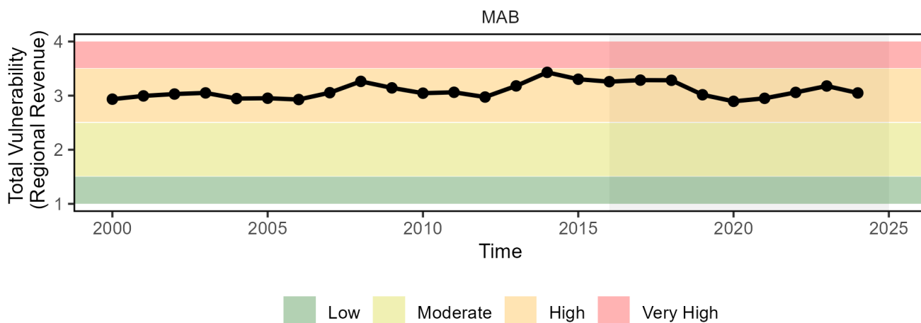
Figure 15: Mid-Atlantic region total vulnerability of commercial revenue (sum of Mid-Atlantic port revenue weighted by species vulnerability scores). Horizontal colored bars show different environmental variability risk levels.
