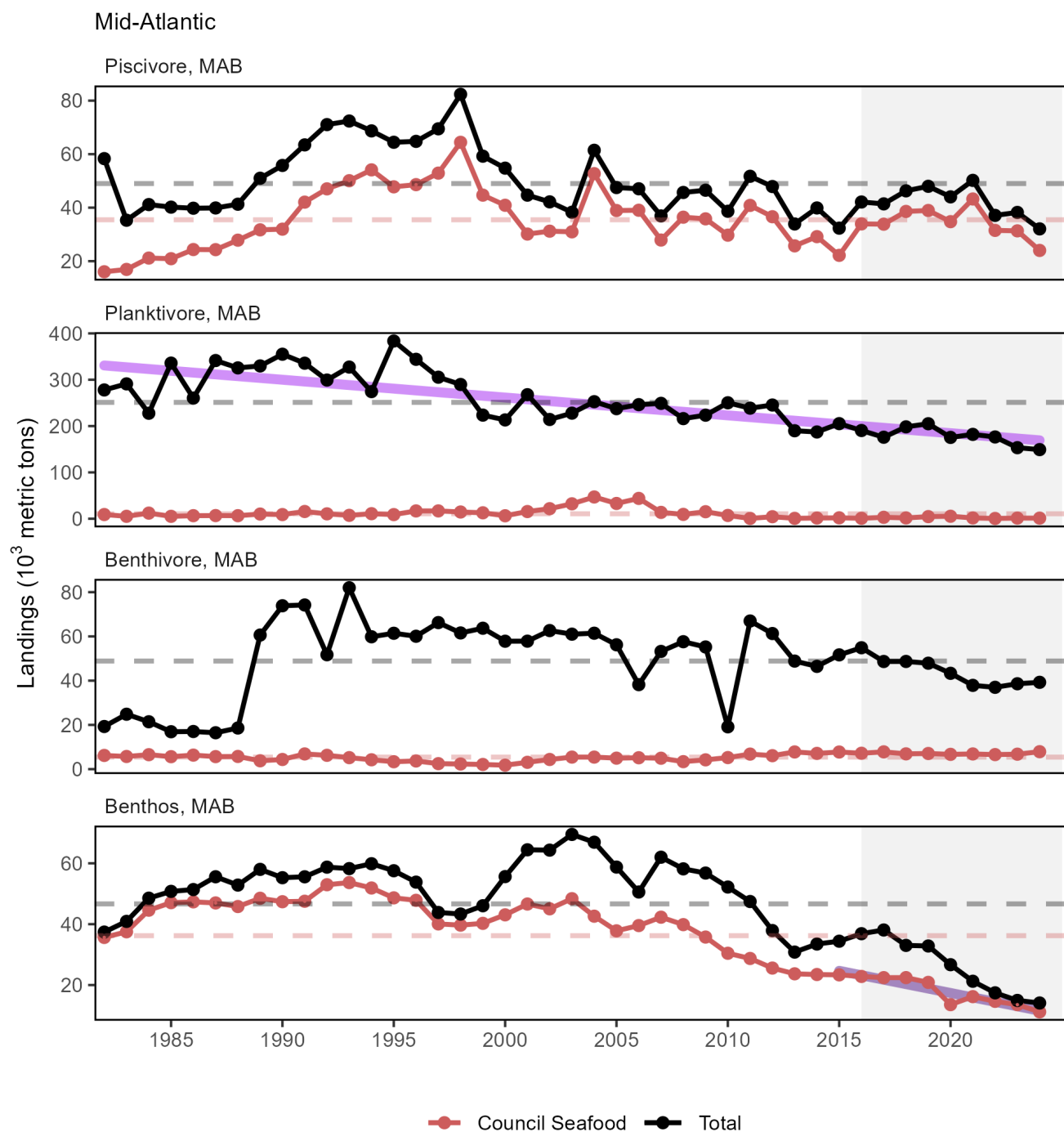
Figure 3: Total commercial landings in the Mid-Atlantic Bight (black) and Mid-Atlantic Fishery Management Council-managed U.S seafood landings (red) by feeding guild, with significant long-term declines (purple) in total planktivore landings and short-term declines (dark purple) in benthos landings.
