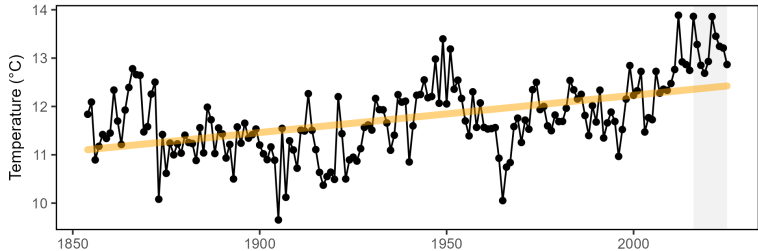
Long-term SST
