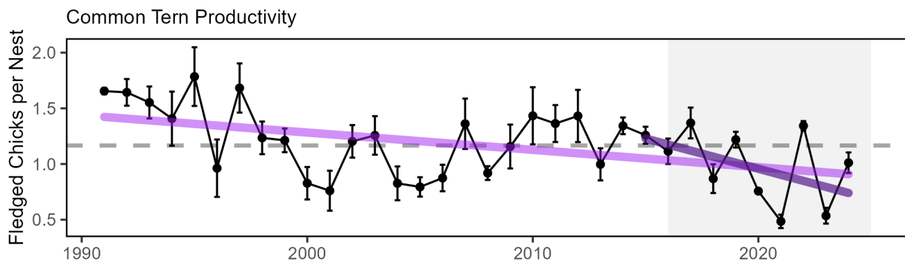
Figure 51: Common tern productivity - the number of fledged chicks per nest - at seven Gulf of Maine colonies managed by the National Audubon Society's Seabird Restoration Program, with significant long-term (purple) and short-term (dark purple) declines.
