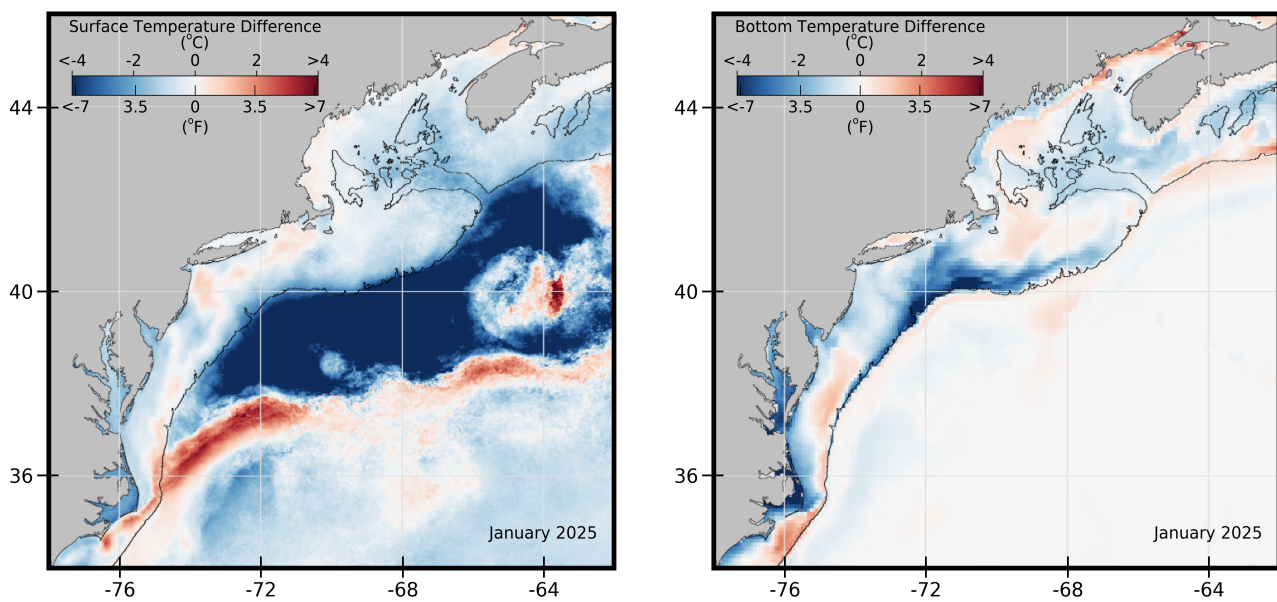
Figure 68: January 2025 sea surface (left) and bottom (right) temperature differences compared to the January climatological means. Sea Surface Temperature (SST) is from the NOAA Advanced Clear-Sky Processor for Ocean (ACSPO) Super-collated SST (climatology range 2000-2020); Bottom temperature is from the GLORYS reanalysis model (climatology range 1990-2020).
