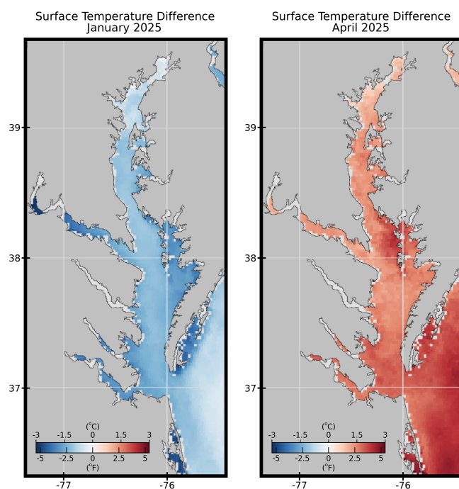
Figure 66: January 2025 (left) and April 2025 (right) sea surface temperature differences compared to the respective monthly climatological means. Sea Surface Temperature (SST) is from the NOAA Advanced Clear-Sky Processor for Ocean (ACSP) Super-collated SST (climatology range 2000-2020).
