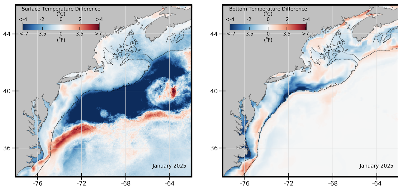
Figure 63: January 2025 sea surface (left) and bottom (right) temperature differences compared to the January climatological means. Sea Surface Temperature (SST) is from the NOAA Advanced Clear-Sky Processor for Ocean (ACSPO) Super-collated SST (climatology range 2000-2020); Bottom temperature is from the GLORYS reanalysis model (climatology range 1990-2020).
