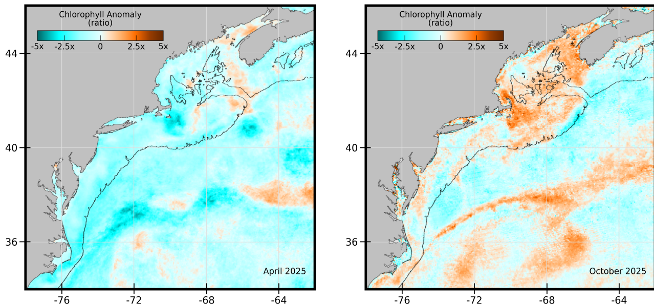
Figure 65: Chlorophyll anomalies shown as the ratio of the monthly concentration compared to the climatological mean (1998-2020) for April (left) and October (right), 2025.
