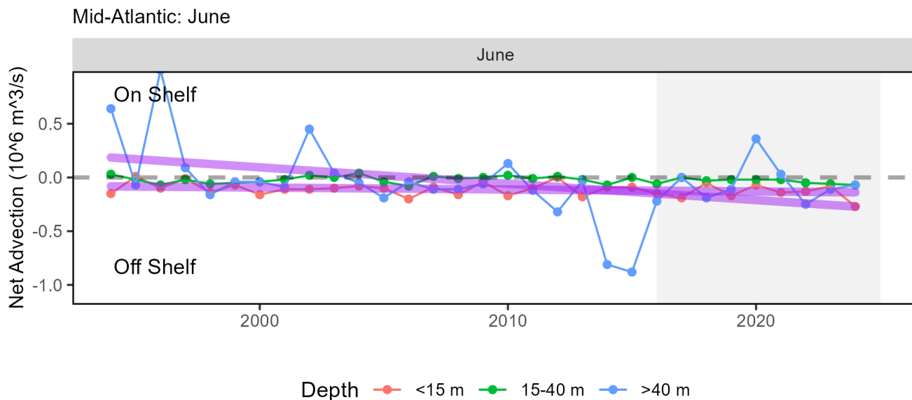
Figure 55: Net advection in June across the Mid-Atlantic continental shelf break within 3 depth bands.
