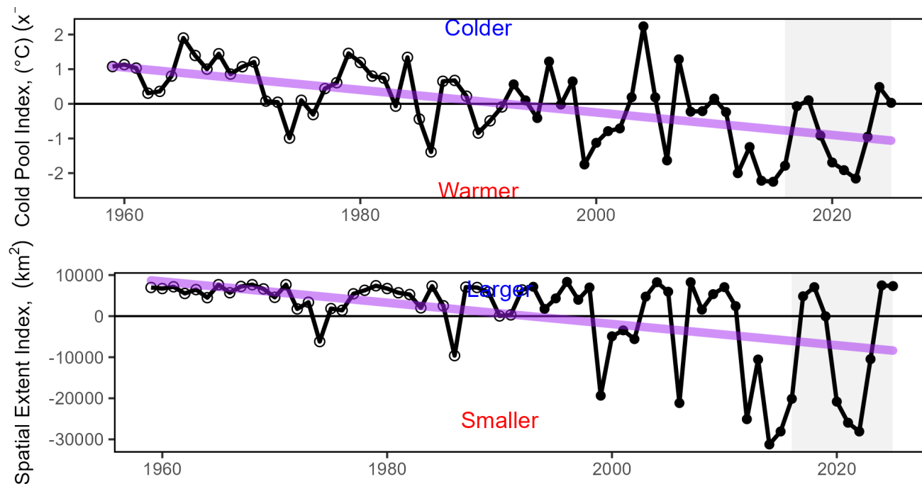
Figure 43: Seasonal cold pool mean temperature (top) and spatial extent index (bottom), based on bias-corrected ROMS-NWA (open circles) and GORYS (closed circles), with declining trends (purple).
